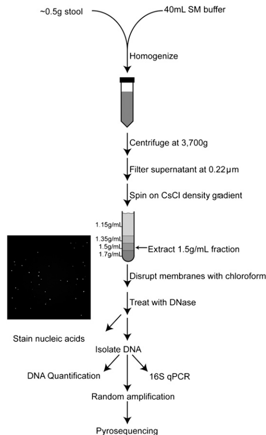
Figure 1. Purification of VLP DNA. Stool was homogenized in SM Buffer; particulate matter was spun down; supernatant was filtered at 0.22 \mu\text{m} to remove cells; VLPs were purified on a CsCl density gradient and treated with nuclease to eliminate unprotected DNA. The absence of bacterial cells was confirmed by staining VLP preparations for nucleic acids. VLP DNA was quantified, amplified, and pyrosequenced.
