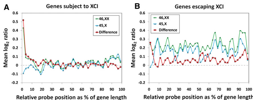
Figure 2. Methylation patterns of genes subject to and escaping X inactivation on active and inactive X chromosomes. (A) For genes subject to XCI, methylation differences between 46,XX and 45,X individuals occur specifically at gene promoters, with 46,XX individuals showing increased methylation compared to 45,X cases. As 83% of RefSeq transcripts listed on the X chromosome have a CGI within 1 kb of their TSS and CGIs are heavily methylated on the X_i versus the X_a , this enrichment of methylation at gene promoters on the X_i is a correlate of CGI methylation. (B) In contrast, for genes escaping XCI, there is a generalized increase in methylation in the bodies of genes in both 45,X and 46,XX individuals compared to genes subject to XCI, with the biggest difference between 46,XX and 45,X occurring at the promoter region. Additionally, a slight but consistent increase in methylation in the bodies of genes escaping XCI is evident in 46,XX compared to 45,X individuals. Two hundred sixteen RefSeq genes listed on chrX scored as subject to XCI (score = 0) and 52 RefSeq genes scored as escaping XCI (score = 8 or 9) by Carrel and Willard (2005) were analyzed. Where multiple splice forms were listed for a single gene, we chose the maximal boundary of all isoforms to define the transcribed region. Probes were then assigned into one of 40 bins depending on their relative position along the gene body, defined by the maximal transcription start and end coordinates. Similar data were observed when considering only those genes of intermediate length (10–100 kb) (Supplemental Figs. 11, 12).
