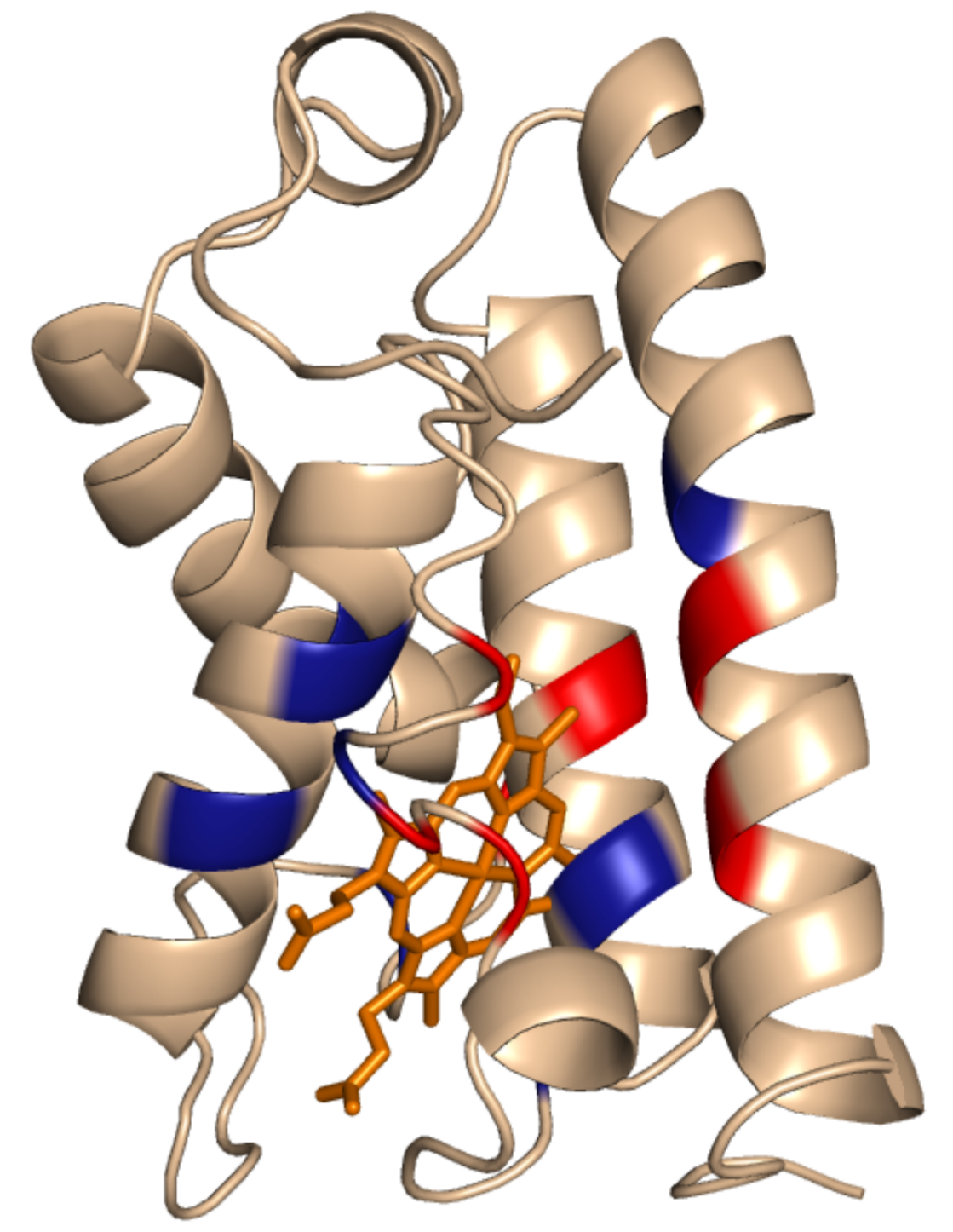
C. Rosetta Model and 1DLWa heme
