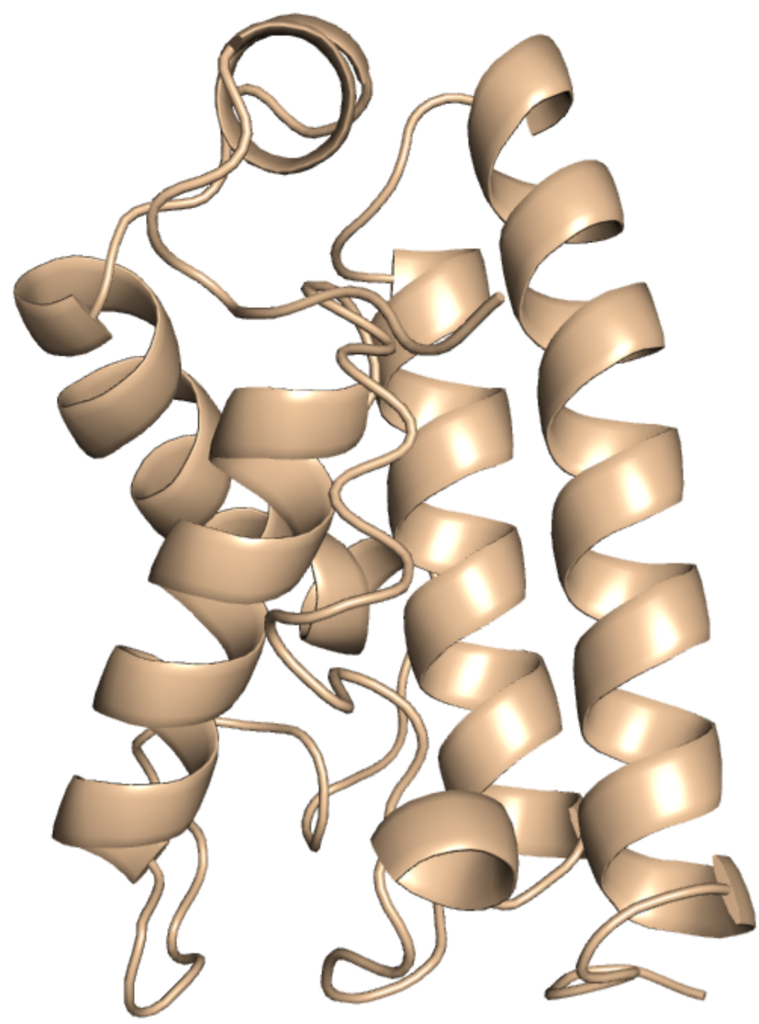
A. Rosetta model of CC_3056
