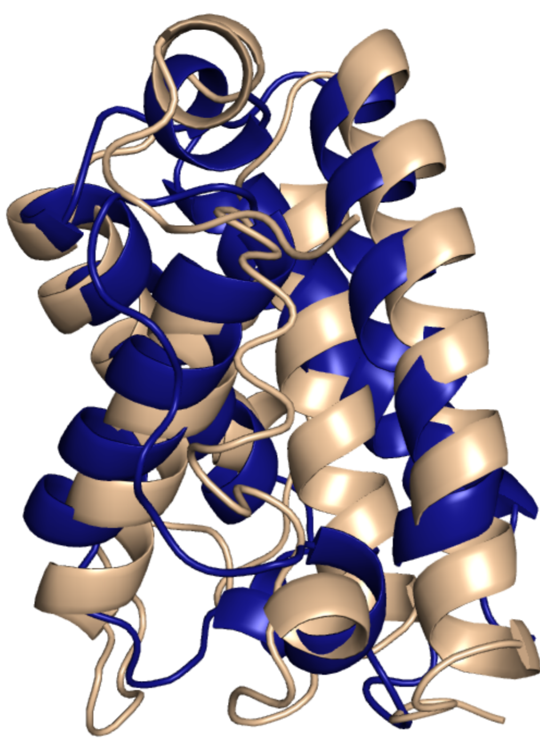
B. Structural alignment w/ 1DLWa
