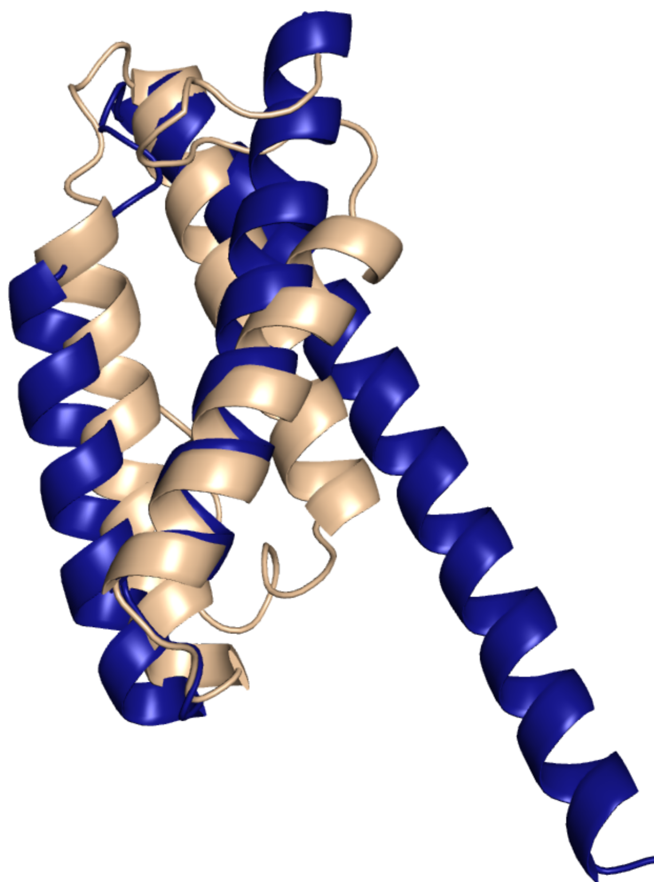
E. Structural alignment w/ 1ECMa
