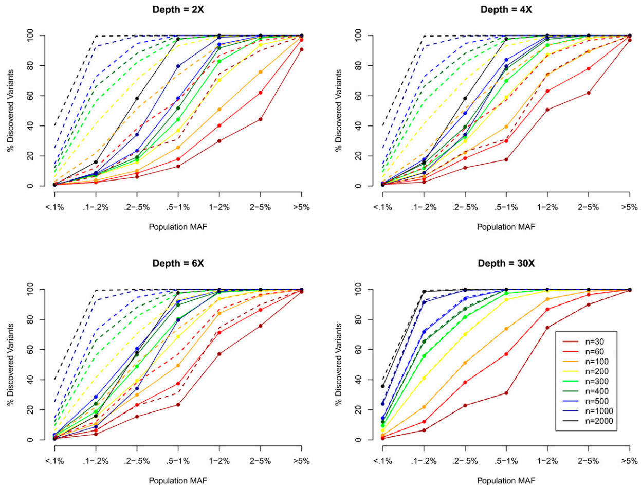
Figure 1. SNP discovery (%) by MAF, sequencing depth, and sequencing sample size. We simulated 30–2000 individuals sequenced at depths 2 \times , 4 \times , 6 \times , and 30 \times . We plotted the % of SNPs discovered by population MAF category (<0.1% to >5%), where population MAF is for the 45,000 simulated chromosomes. The dotted lines show the % of SNPs in each population MAF category that is polymorphic among the sequenced individuals.
