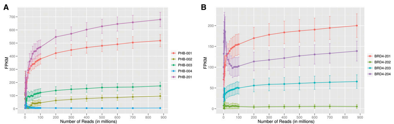
Figure 6. Expression levels versus sequencing depth. We plotted FPKM values for genes and their transcripts at various sequencing depths. (A) FPKM values of five spliced forms of PHB are shown; the least abundant isoform (blue line) of PHB reaches within 20% of its “final” FPKM value with only 60 million reads; however, the expression values of the other four isoforms continued to increase with more reads. (B) FPKM values of BRD4 are shown. With less than 100 million reads, the expression level of BRD4-201 (orange line) is overestimated, while that of BRD4-204 (purple line) is underestimated. (Error bars represent 95% confidence intervals.)
