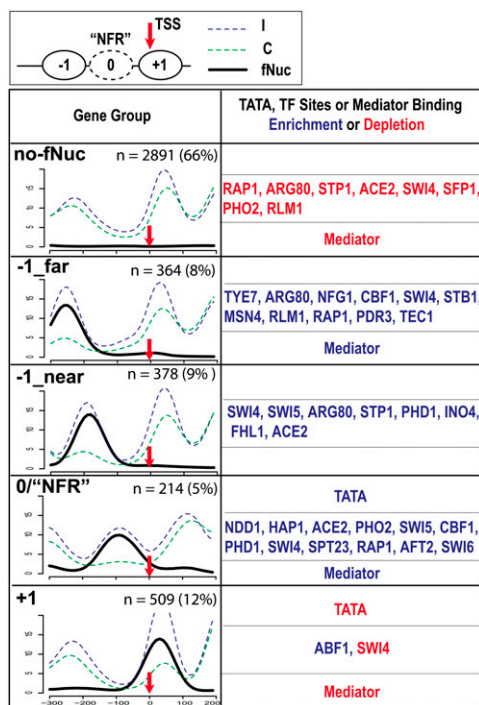
Figure 2. Classification of RNAP II genes into five groups by K-means clustering based on fragile nucleosome occupancy in promoters. ( Upper ) A diagram illustrating the canonical nucleosomal organization at the promoter. TSS (red arrow): transcription start site; ovals labeled with +1 and -1 are nucleosomes on or upstream to TSS. Oval in dashed line (0) is the fragile nucleosome at the NFR. The “Gene Group” column depicts the overlay of nucleosome distribution of all the genes in each group. Group names, based on the fragile nucleosome position, are in bold at upper left corners. ( x -axis) The nucleotide positions, with TSS = 0. ( y -axis) The normalized number of sequencing counts. (Blue) Incomplete digestion; (green) complete digestion; (black) differential signals representing fragile nucleosome; ( n ) numbers of genes in each group; the percentage indicates the portion of total characterized genes. Enrichment and depletion of TATA, TF sites, and mediator binding are marked by blue and red, respectively. The P -value cutoff for TF binding site enrichment is 1.0 \times 10^{-10} .
