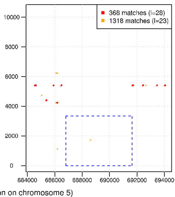
Fixed-length seeds
