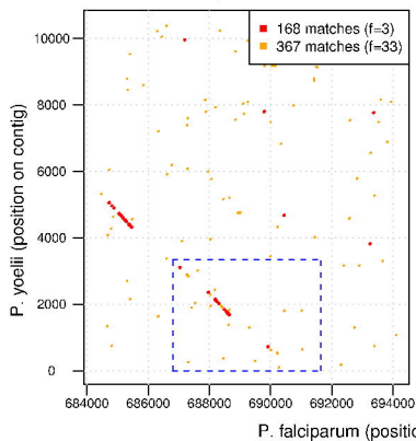
Adaptive seeds
