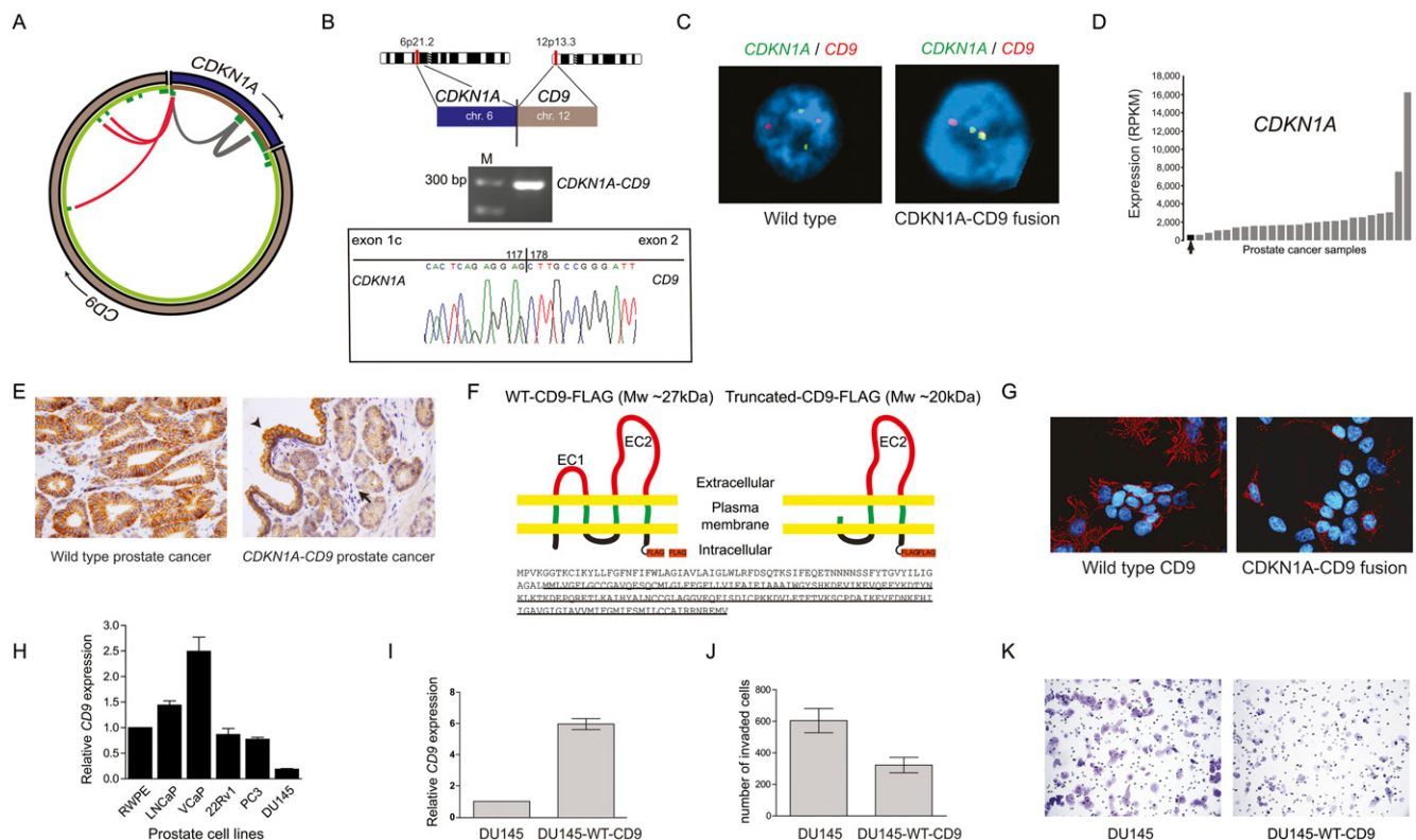
Figure 3. Characterization of the CDKN1A – CD9 gene fusion candidate. (A) Mapping of PE RNA-seq reads to CDKN1A with either both ends mapping to CDKN1A (gray) or one end mapping to CD9 (red) and thereby connecting CDKN1A exon 1 to 3' exons of CD9 . (B) Experimental validation of the gene fusion transcript by RT-PCR and subsequent Sanger sequencing. (C) FISH validation of the CDKN1A – CD9 fusion in the index case (right) but not in another control cancer (left). (D) The fusion positive prostate cancer sample (black) has the lowest CDKN1A expression levels across 25 prostate cancers. Expression levels are indicated in reads per kilobase of exon model per million mapped reads (RPKM) as defined previously (Mortazavi et al. 2008). (E) Immunohistochemistry of CD9 in prostate cancer. (Left) Strong CD9 membranous expression detected in malignant glands from a prostate cancer sample without a detectable CD9 rearrangement. (Right) Malignant glands in CDKN1A – CD9 fusion positive case (arrow) showing weak membranous expression in comparison to adjacent benign areas (arrowhead). (F) Schematic illustration of Flag-tagged WT-CD9 and Flag-tagged CDKN1A – CD9 fusion protein. The fusion event leads to a truncated CD9 protein with loss of two transmembrane domains and the small extracellular domain (EC1). (Bottom) The amino acid sequence of WT-CD9 protein with the truncated CD9 protein version underlined. (G) Immunofluorescence staining revealed the expression of WT-CD9 and truncated CD9 in HEK293 cells stained with anti-Flag (red) antibody. Nuclei were stained with DAPI (blue). (H) Expression levels of CD9 mRNA transcripts in prostate cell lines. (I) CD9 expression from control or stably CD9 -expressing DU145 cells. (J) Bar graph comparing the invasiveness of the two lines as assessed by Boyden chamber assays. (K) Representative images of invaded cells for each cell line.
