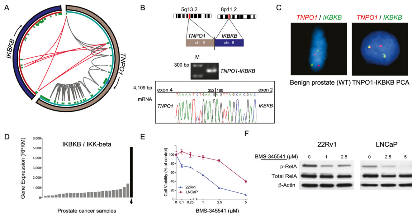
Figure 4. Characterization of the TNPO1 – IKBKB gene fusion candidate. (A) Mapping of PE RNA-seq reads to TNPO1 with either or both ends mapping to TNPO1 (gray) or one end mapping to IKBKB (red). (B) Experimental validation by RT-PCR and Sanger sequencing verifies the expression of a TNPO1 – IKBKB fusion transcript. (C) Fusion specific FISH assays confirm the existence of TNPO1 – IKBKB fusion in cancer tissue (right) but not in adjacent benign tissue (left). (D) IKBKB expression levels in a set of 25 prostate cancers. IKBKB levels are highest in the fusion positive sample (black). (E) Dose response curve assessing the effect of the IKK-beta inhibitor BMS-345541 on viability of LNCaP and 22Rv1 prostate cancer cells. (F) Immunoblots depicting the effect of BMS-345541 exposure on RelA phosphorylation in LNCaP and 22Rv1 cells.
