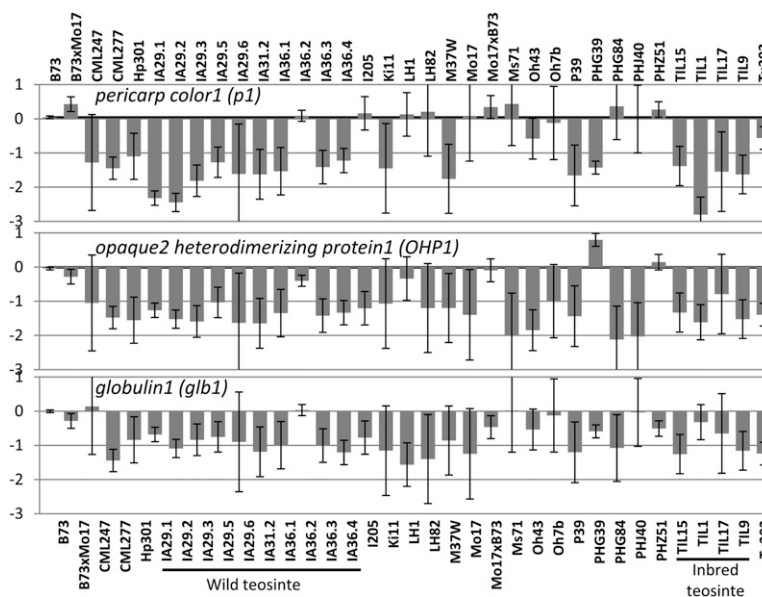
Figure 5. Examples of CNV for previously characterized maize genes. The CGH data are summarized for three maize genes. For each genotype the average \log_2 ratio for all probes from the gene is summarized as the height of the bar, and the standard deviation for the multiple probes is represented by the error bars.
