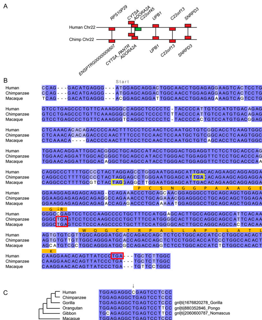
Figure 3. Sequence changes in the origin of C22orf45 from noncoding DNA. As in Figure 2: (A) Region of conserved syntenic between human and chimp chromosomes 22. One gene in this region, C22orf45 , had no BLASTP hits in any other genome and is shown in green. (B) Multiple sequence alignment of the gene sequence of C22orf45 and similar nucleotide sequences from the syntenic location in chimp and macaque. The arrow indicates the location of an in-frame stop codon shared by chimp and macaque that would result in premature termination (red box) irrespective of the other disablements. The codons highlighted with a yellow box indicate the stop codon including all disablements (indels) in chimp and macaque for the reading frame starting from the same location as the human start (note the ATG start codon is absent in macaque and that the frameshifts mean the hypothetical protein sequence is drastically altered). (C) The disabler is also shared by gorilla, orangutan, and gibbon indicating it is ancestral.
