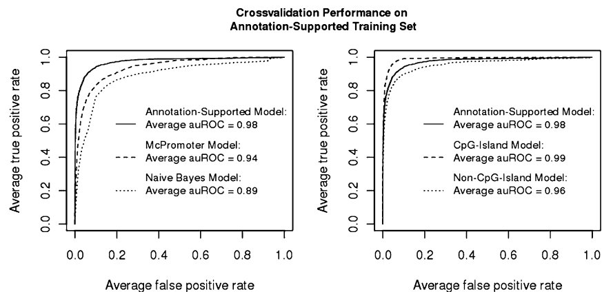
Figure 4. Tenfold cross-validation performance comparisons for the annotation-supported model. (Left) The plot compares the performance of two additional classifiers, a naive Bayes classifier and McPromoter's HMM classifier. (Right) The plot compares CpG-island and non-CpG-island models. ROC curves with threshold averaging are displayed in both plots, along with the average area under the curve (auROC). Positive examples are the experimentally supported CAGE single-peak TSS locations, while negative examples are selected from intergenic and coding regions (see Fig. 3B).
