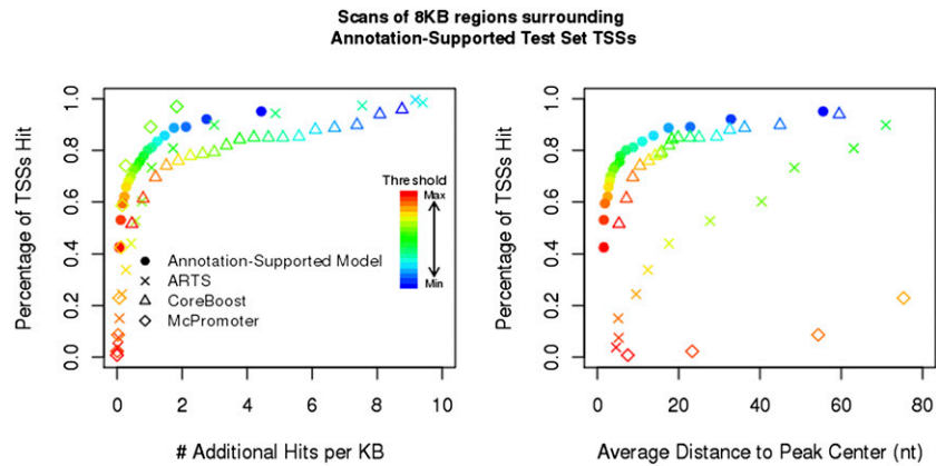
Figure 5. Performance on scans of the annotation-supported test set. ( Left ) The case in which a TSS is considered to be a hit if a probability peak contains the TSS. The curve represented by each symbol type shows the percentage of TSS hit as a function of the number of additional hits per kilobase. ( Right ) Each curve displays the average distance to the center of the probability peak computed over all of the peaks containing a TSS. At each threshold value (color), the plots give a comparative view of how many additional peaks are being called versus how well the TSS-containing peaks approximate actual TSS location.
