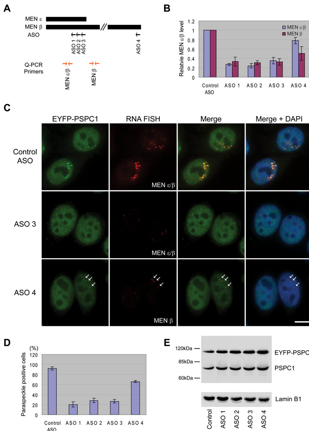
Figure 5. The MEN \epsilon/\beta transcripts are essential for the integrity of nuclear paraspeckles. (A) Antisense oligonucleotides (ASO) were designed to knock down MEN \epsilon/\beta or MEN \beta expression in HeLa cells. Three ASOs (ASO 1, 2, and 3) target both MEN \epsilon and \beta isoforms, while ASO 4 targets only the MEN \beta transcript. (Arrows) The positions where each ASO targets the MEN \epsilon/\beta transcripts. (B) Twenty-four hours after transfection of ASOs into HeLa cells stably expressing EYFP-PSPC1 (also known as PSP1 \alpha ), an ~70% knockdown of MEN \epsilon/\beta (ASO 1, 2, or 3) or 50% knockdown of MEN \beta (ASO 4) was achieved, as assessed by Q-PCR. Beta-actin was used as a normalization control. The data in the histogram are shown as mean and standard deviation values of three independent experiments. (C) RNA FISH was performed 24 h after HeLa EYFP-PSPC1 cells were transfected with a control ASO or ASOs targeting the MEN \epsilon/\beta or \beta transcript, to identify cells in which the RNAs were knocked down. In cells transfected with the control ASO, MEN \epsilon/\beta transcripts are localized to paraspeckles. Cells transfected with ASO 3 or 4 did not show paraspeckles. (Arrows) Residual paraspeckles in a cell where knockdown of the MEN \beta transcript was not complete. Scale bar, 10 \mu m. (D) The portion of paraspeckle-positive cells was reduced to ~20% by ASO 1, 2, or 3, while control ASO did not appear to influence the integrity of paraspeckles. Treatment with ASO 4 resulted in a loss of paraspeckles, although to a lesser extent. The data in the histogram are shown as mean and standard deviation values of three independent experiments. Approximately 100 cells were counted per experiment. (E) Knockdown of the MEN \epsilon/\beta transcripts did not result in degradation of the PSPC1 protein. Lamin B1 serves as a loading control.
