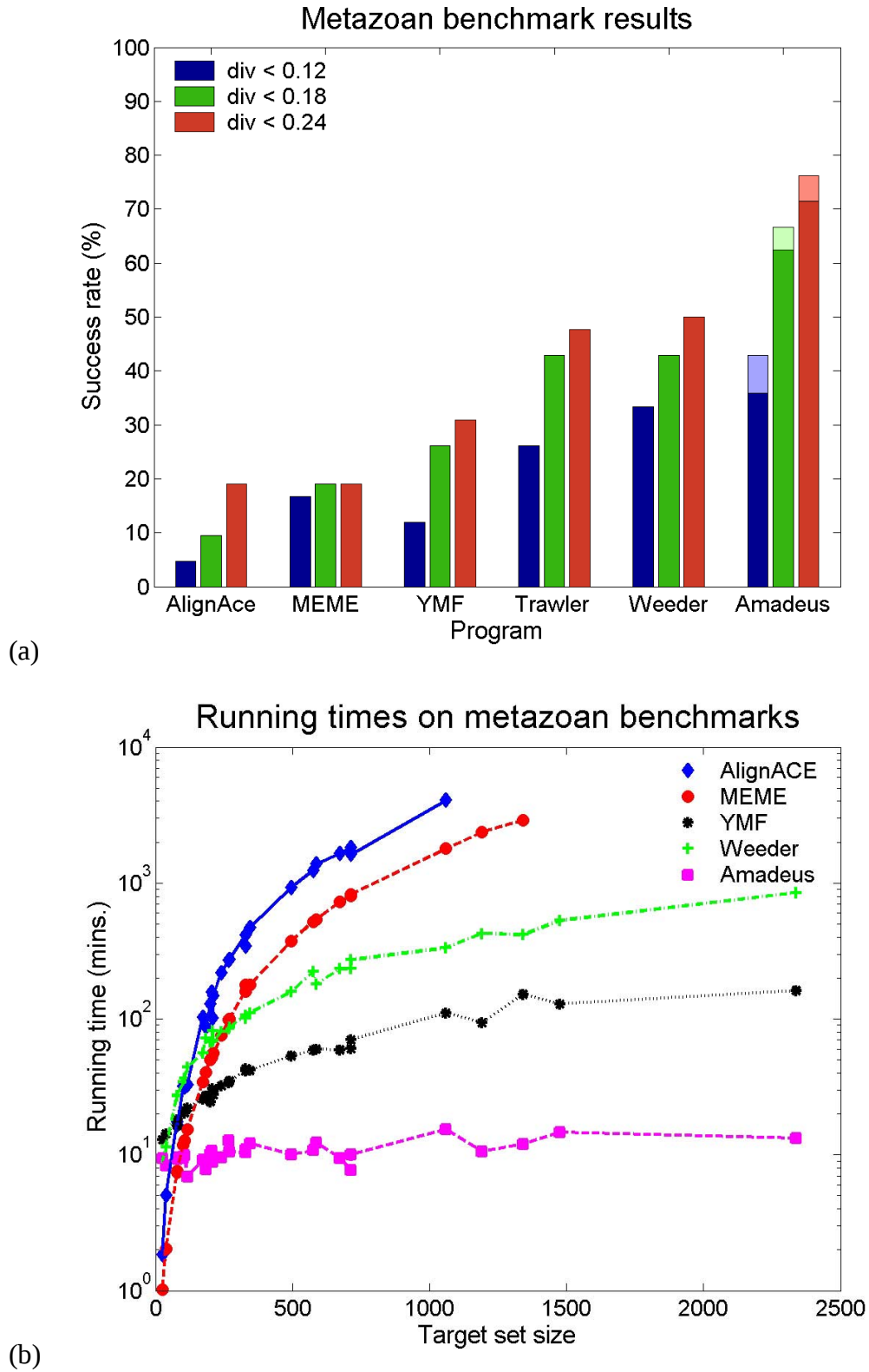
Figure 4. Performance of six motif finding tools on our compendium of metazoan target sets.
