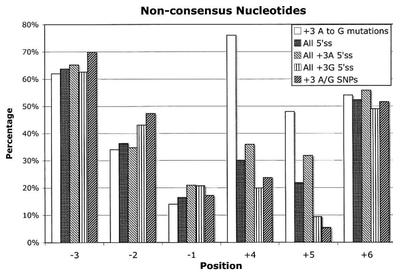
Figure 4. Percentage of nonconsensus nucleotides at positions (X-axis) of the 5'ss for five classes of 5'ss: all 5'ss in human (186,630 cases), 5'ss with A at +3 (110,598), 5'ss with G at +3 (64,837), 5'ss with SNPs having alleles A/G at position +3 (93), and 5'ss with disease-causing A-to-G mutations at +3 (50 cases). 5'ss with disease-associated A-to-G mutations at position +3 tend to have nonconsensus nucleotides at positions +4 and +5 more frequently than the other sets, which suggests their disruptive nature, based on the association matrix (Fig. 2).
