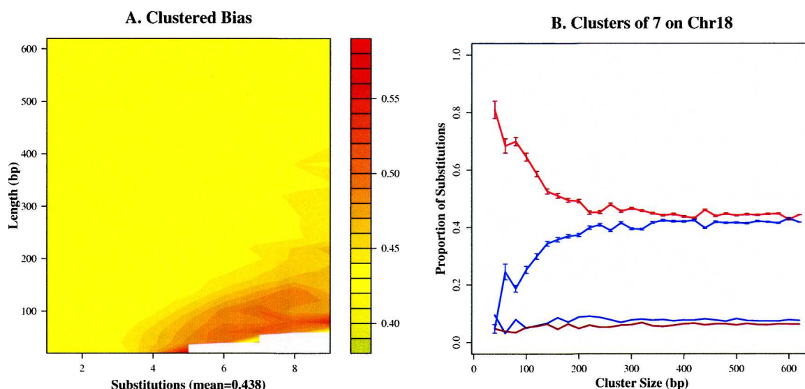
Figure 1. Clusters of substitutions are biased weak (AT) to strong (GC). (A) This heat map shows the proportion of substitutions that are weak-to-strong (color scale) as a function of the local substitution rate for a range of sizes and densities of substitutions. The overall proportion of substitutions that are weak-to-strong is 0.438 genome-wide (yellow). As substitution density approaches 4 or more within 100 bp, the proportion rises to 0.58 (red). (B) Chromosome 18 shows a particularly strong relationship between substitution density and bias, as can be seen for clusters of seven substitutions in the “zipper” plot. A similar pattern was observed on all autosomes. Additional graphics are available at http://www.soe.ucsc.edu/research/compbio/ubcs/ .
