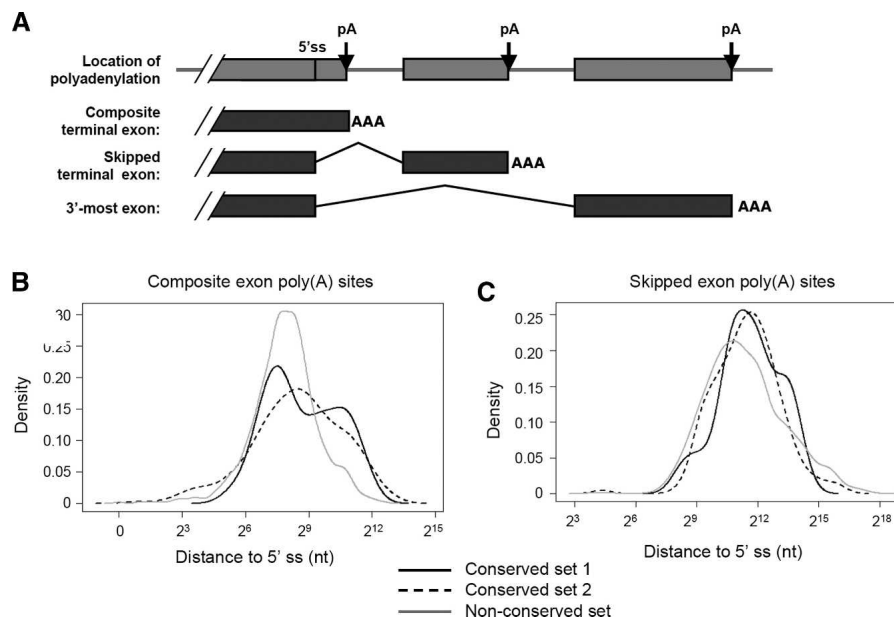
Figure 1. Intronic poly(A) sites in human genes. (A) Schematic of poly(A) sites located in different types of exons, i.e., composite terminal exon, skipped terminal exon, and 3'-most exon. 5'ss indicates 5' splice site; pA, poly(A) site. Exons are shown as boxes. Splicing is indicated by an angled line. (B) Distance between 5'ss and composite exon poly(A) sites. Median values are 295 nt, 355 nt, and 238 nt for poly(A) sites in the conserved set 1, conserved set 2, and nonconserved set, respectively. (C) Distance between 5'ss and skipped exon poly(A) sites. Median values are 3445 nt, 2997 nt, and 2320 nt for poly(A) sites in the conserved set 1, conserved set 2, and nonconserved set, respectively. As indicated, solid black lines are for poly(A) sites in the conserved set 1, dotted black lines are for poly(A) sites in the conserved set 2, and solid gray lines are for poly(A) sites in the nonconserved set.
