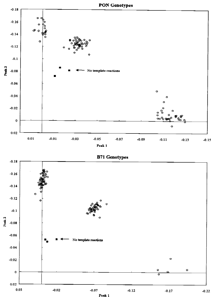
Figure 3 Cluster analysis. From the melting profile of each sample is plotted its peak 1 and peak 2 areas, as detailed in the text. (○) Genomic DNA containing samples; (■) no-template controls.
