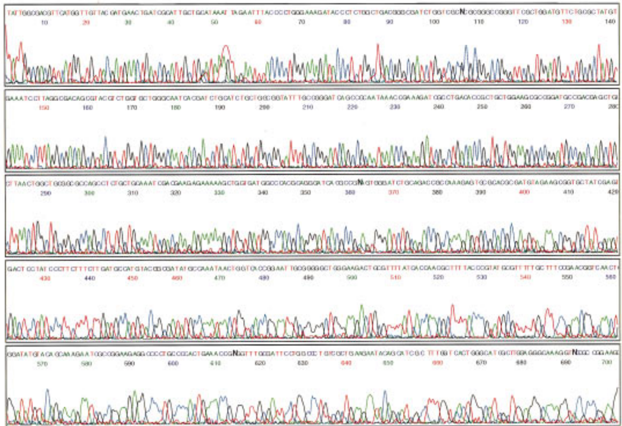
Figure 1 Sequencing of E. coli K12 strain genomic DNA with BigDye terminators. Approximately 3 \mu g of E. coli DNA was sequenced with an apaG gene primer (5'-GTTCCCACTCATTTCATTA) using the conditions described in the text.
