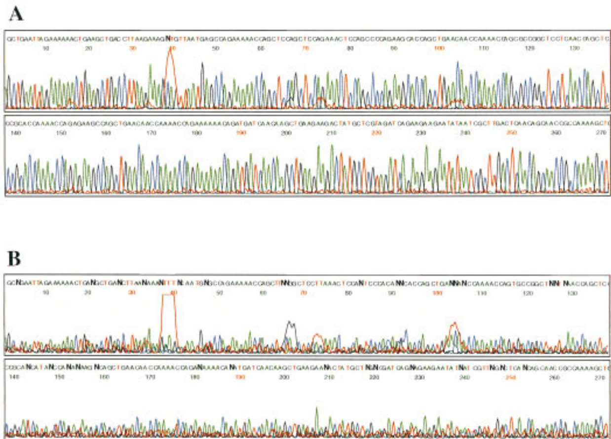
Figure 2 Sequencing of S. pneumoniae genomic DNA with BigDye terminators using either 2.5 \mu g (A) or 5.0 \mu g (B) of template and a SKH1 primer (23-mer 5'-AACAAATAATGTAGAAGACTACTT). All other conditions are as described in the text.
