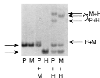
Figure 2 A silver-stained native polyacrylamide (8%) gel showing the separation of a 150-bp PCR product of the PAX8 gene amplified from pig (P), mouse (M), and human (H) genomic DNA; P + M, P + H, and M + H were mixed subsequent to the PCR amplification but prior to the denaturation/renaturation treatment. Homo- and xeno-duplexes are marked by arrows to the left and right , respectively.
