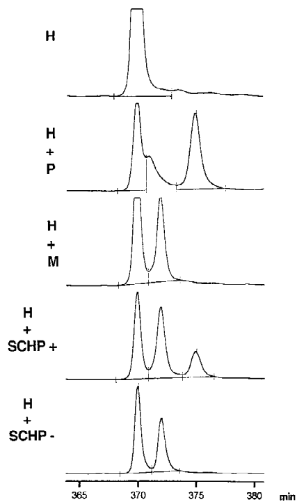
Figure 3 Electropherogram showing the separation of a 157-bp PCR fragment of the HOXD gene in a 8% native polyacrylamide gel by use of a DNA sequencing instrument (ALF Express, Pharmacia Biotech). HOXD was amplified from human (H), pig (P), mouse (M), one pig/mouse SCH clone containing the pig HOXD gene (SCHP+), and one clone negative for the pig HOXD gene (SCHP-). Only the human product was amplified by use of fluorescently labeled primers and this product was added to the other amplification products prior to the denaturation/renaturation treatment. As a consequence, only human homoduplexes and human/mouse and human/pig xenoduplexes were visualized.
