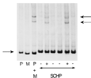
Figure 1 A silver-stained native polyacrylamide (8%) gel showing the separation of a 333-bp PCR product of the PKLR gene amplified from pig (P), mouse (M), and six clones from a pig/hamster SCH panel; P + M was mixed subsequent to the PCR amplification but prior to the denaturation/renaturation treatment. Homo- and xenoduplexes are marked by arrows to the left and right , respectively. SCH clones that were scored positive and negative for the pig PKLR gene are marked by + and –, respectively.
