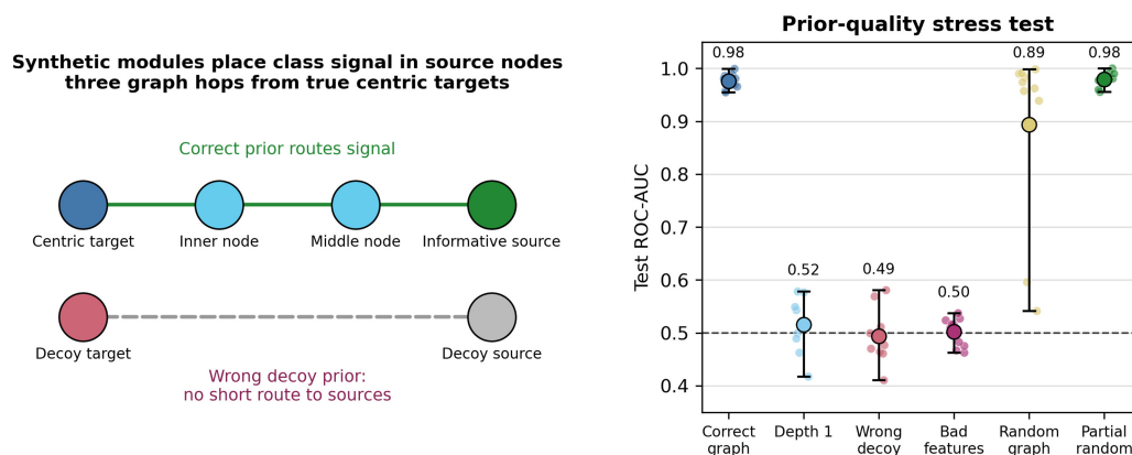
Figure 5. Controlled prior-robustness simulation design and summary. Informative source nodes were placed three graph hops from true centric targets in pathway-like modules, and decoy targets were placed in separate modules. Performance under the correct graph prior is high and stable, whereas a wrong decoy graph and fully bad centric features are near chance. The random graph condition has larger variability because it can occasionally route true source nodes by chance.
