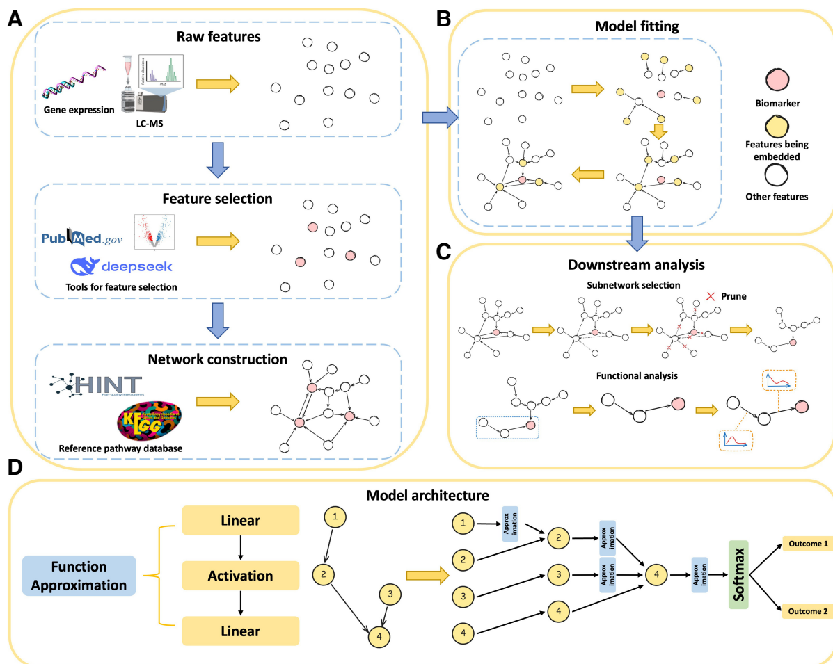
Figure 1. Overview of the PathNet workflow and model architecture. (A) Raw molecular features are acquired from omic platforms such as gene-expression profiling and LC–MS; candidate centric features are selected using biological knowledge and data-driven evidence; and pathway or interaction databases are used to construct the local prior graph around those centric features. (B) During model fitting, pathway-connected neighboring features are embedded toward selected biomarker/centric features through sparse graph-constrained connections, whereas unrelated features are excluded from the corresponding local propagation route. (C) After training, retained edge functions are used for downstream analysis, including subnetwork selection by pruning weak connections and functional analysis of learned edge-specific response curves. (D) The model architecture uses edge-specific functional approximation blocks and a sparse feed-forward propagation structure before the final softmax prediction layer.
