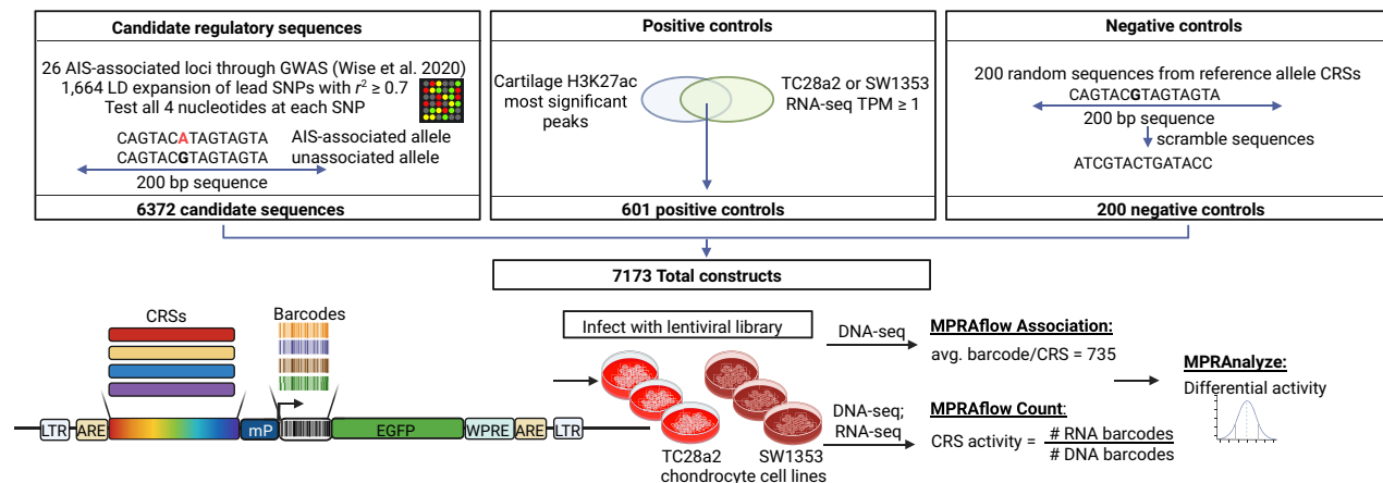
Figure 1. Overview of the MPRA design. This schematic shows the selection process of choosing the candidate regulatory sequences to be investigated in the assay (top left), selection of positive controls (top middle), and negative controls (top right). Bottom panel shows an overview of the MPRA steps, including the segment of DNA that is integrated into the cell genome (left), transduction into chondrocyte cell lines (middle), and the downstream sequencing and processing of the MPRA (right).
