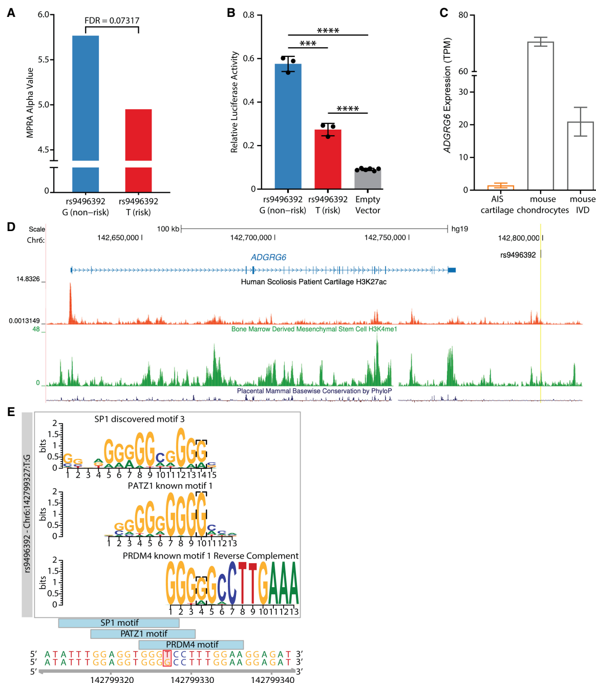
Figure 4. Predicted transcriptional disruption owing to variant rs9496392. (A) MPRA signal of rs9496392 CRS in TC28a2 ( n = 3 ). The reported false-discovery rate (FDR) value is a FDR adjusted likelihood ratio test P -value of the difference in activity between alleles reported by MPRAalyze. (B) Relative luciferase activity of the rs9496392 CRS in TC28a2 ( n = 3 ). (*** P < 0.001 ; (****) P < 0.0001 ). The statistical significance between CRS activity and empty-vector negative controls was determined by one-way ANOVA; the statistical significance between SNP alleles was determined by unpaired Student's t -test. (C) Expression of ADGRG6 in AIS spinal cartilage, mouse chondrocytes, and mouse intervertebral disc. (D) Scoliosis H3K27ac ChIP-seq (red) and mesenchymal stem cell-derived chondrocyte H3K4me1 (green) enrichment at the rs9496392 enhancer (highlighted in yellow). (E) Predicted disruption of transcription factor binding motifs. Error bars indicate mean \pm SD.
