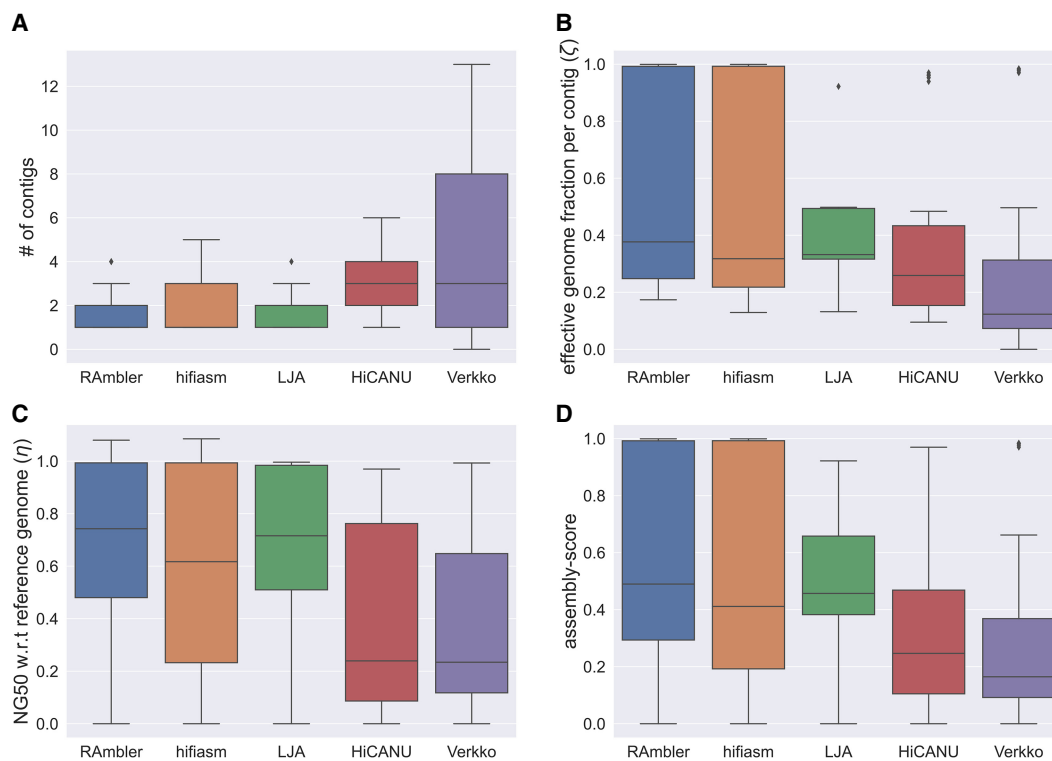
Figure 2. Assembly statistics for RAMbler, hifiasm, LJA, HiCANU, and Verkko for 36 different combinations of synthetic data with repetitive regions having repeat sizes \{15, 20\} kb, number of copies \{5, 10\} , mutation rate P = \{1/250, 1/500, 1/1000\} , and coverage depth \{20\times, 30\times, 40\times\} . (A) Number of contigs, (B) effective genome fraction per contig \zeta , (C) normalized NG50 \eta , and (D) assembly score.
