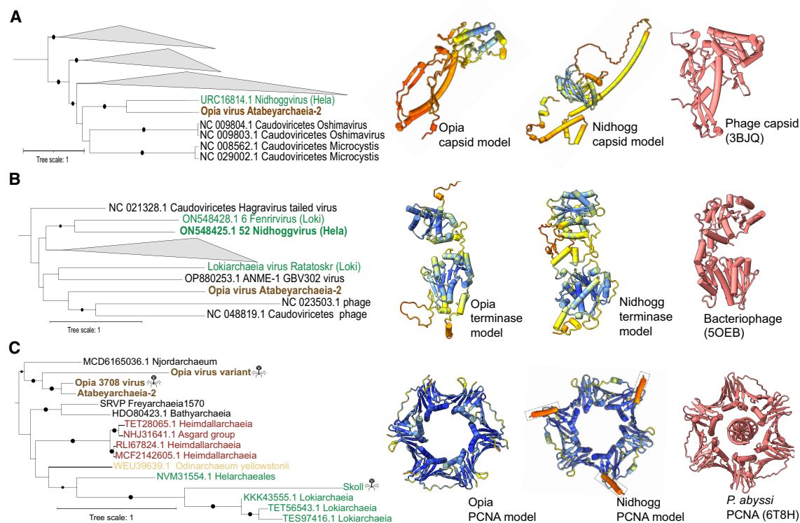
Figure 4. Evolutionary relationships and structural conservation of Opia virus hallmark proteins. (A–C) Maximum-likelihood phylogenetic trees of capsid (A), terminase large subunit (B), and proliferating cell nuclear antigen (PCNA; C). Trees are midpoint-rooted; circles indicate bootstrap support >70%. Insets show structural models: Opia virus (infecting Atabeyarchaeia, this study) and Nidhogg virus (infecting Helarchaeales) colored by AlphaFold3 confidence (blue to red, high to low), with best FoldSeek match in coral. Reference structures: bacteriophage capsid (PDB: 3BJQ) for A, large terminase from thermophilic bacteriophage D6E (PDB: 5OEB) for B, and P. abyssi PCNA (PDB: 6T8H) for C. Scale bars represent one substitution per site. Opia virus variants cluster with other Asgardarchaeota MGEs, highlighting their evolutionary relationships within this archaeal phylum.
