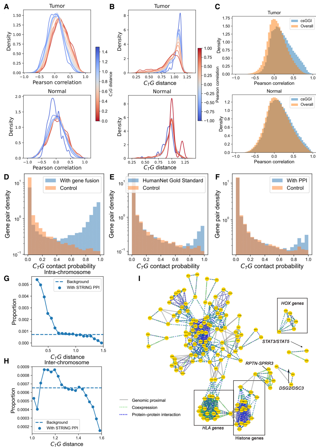
Figure 4. Passage of gene-gene interplay from genomic level to transcription and protein levels in colorectal cancer. (A) The distribution of transcriptional Pearson correlation under different C_{7G} distance of the whole chromosome; the color of each line indicates the corresponding C_{7G} distance. (B) The distribution of C_{7G} distance under different Pearson correlation of the whole chromosome; the color of each line indicates corresponding Pearson correlation coefficient. (C) The distribution of correlation of gene pairs with csGGIs and overall background. (D) Distribution of C_{7G} contact probability for gene pairs with (blue) and without (orange) gene fusion events reported in FusionGDB2 data set. (E) Distribution of C_{7G} contact probability for gene pairs with (blue) and without (orange) similar biological process reported in HumanNet. (F) Distribution of C_{7G} contact probability for gene pairs with (blue) and without (orange) PPIs reported in STRING database (G) The proportion of intra-chromosomal gene pairs with STRING PPI at different C_{7G} distances in the tumor sample. The proportion refers to number of gene pairs with PPIs at fixed C_{7G} distance/number of all gene pairs at fixed C_{7G} distance. The background refers to number of gene pairs with PPIs/number of all gene pairs at all C_{7G} distance. (H) The proportion of inter-chromosomal gene pairs with STRING PPI at different C_{7G} distances in tumor sample. (I) The gene network integrates colon cancer-related gene-gene interplay at the DNA, RNA, and protein levels. The three kinds of edges indicate gene-gene interplays at three levels.
