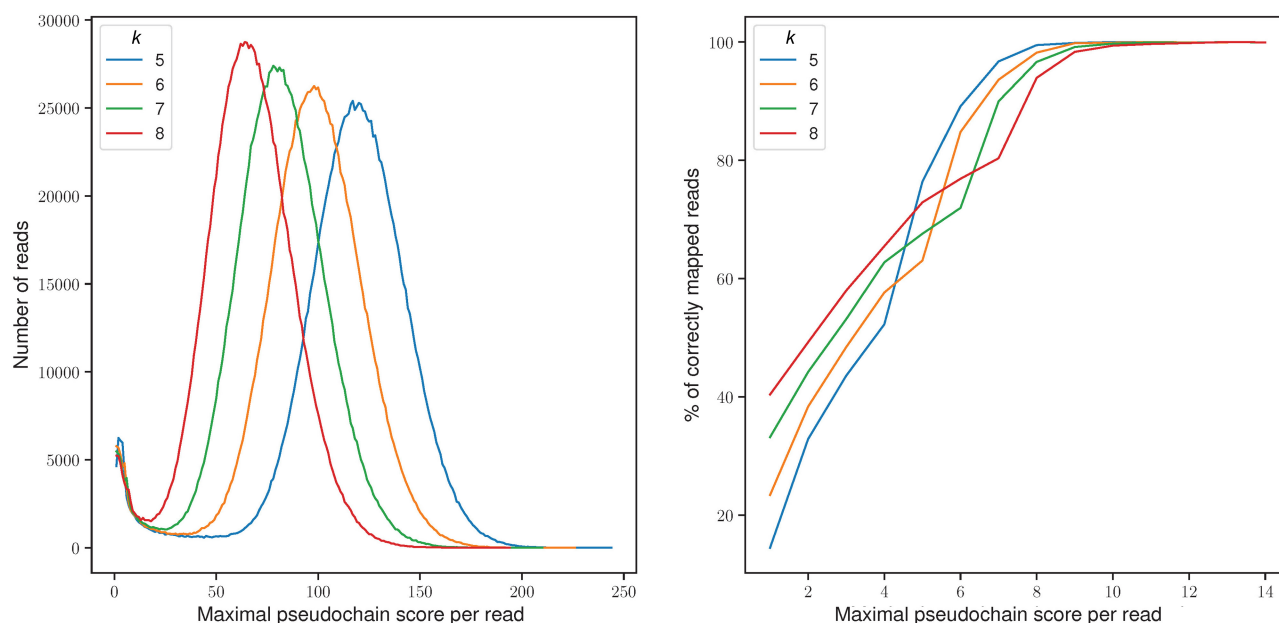
Figure 3. Effect of pseudochain score on mapping accuracy. The x-axis in both subfigures corresponds to the score of the maximal pseudochain per read; on the left , the y-axis denotes the total number of reads with the corresponding maximal pseudochain score; on the right , the percentage of reads that are correctly mapped (assessed by paftools mapeval ) with the corresponding maximal pseudochain score. Only the scores below a threshold s , where s denotes the maximum score at which a read was mapped incorrectly, are plotted. The parameters used for mapquik were k = 5-8 , \ell = 31 , \delta = 0.01 .
