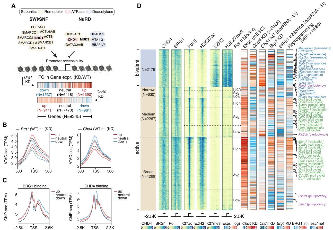
Figure 1. RNA polymerase II (Pol II)-bound genes respond oppositely to that of PRC2-bound genes upon perturbation of SWI/SNF or NuRD activities. (A) The composition of the SWI/SNF and NuRD remodeling complexes. BRG1 (SWI/SNF) and CHD4 (NuRD) are the ATPase subunits of these complexes. SWI/SNF supports open whereas NuRD supports closed chromatin states at gene promoters. Also shown are the SWI/SNF and NuRD target genes in mESCs ( N = 9345 ) binned into groups of 25 each and rank-ordered based on the Pol II binding levels at their promoters. For each bin, the median gene expression fold changes following Chd4 or Brg1 knockdown (KD) are shown. (B) Changes in promoter accessibility at genes that are up-regulated, neutral, or down-regulated following KD of Brg1 (left) or Chd4 (right). Standard error is represented by a shaded area around the lines. (C) BRG1 and CHD4 binding signals at the promoter of genes that are up-regulated, neutral, or down-regulated following KD of Brg1 (left) or Chd4 (right). (D) Occupancy levels of CHD4, BRG1, Pol II, EZH2, and histone modifications (H3K27ac and H3K27me3) at active ( N = 7166 ) and bivalent ( N = 2179 ) gene promoters. Active promoters are further subclassified based on their widths: narrow, \leq 500 bp; medium, 500–1000 bp; broad, > 1000 bp. Genes are binned into groups of 25 each and rank-ordered based on the Pol II binding levels at their promoters. For each bin, the median gene expression fold changes following Chd4 or Brg1 KD or during MEF-to-mESC reprogramming. Also shown are the changes in absolute (spike-in normalized) nascent RNA levels upon BRG1 inhibitor treatment (BRM014 for 3 h) and Chd4 KD. Genes corresponding to the KEGG pathways regulated by high/average Pol II-bound and low Pol II-bound/bivalent genes are marked on the heatmap (Supplemental Fig. S3A).
