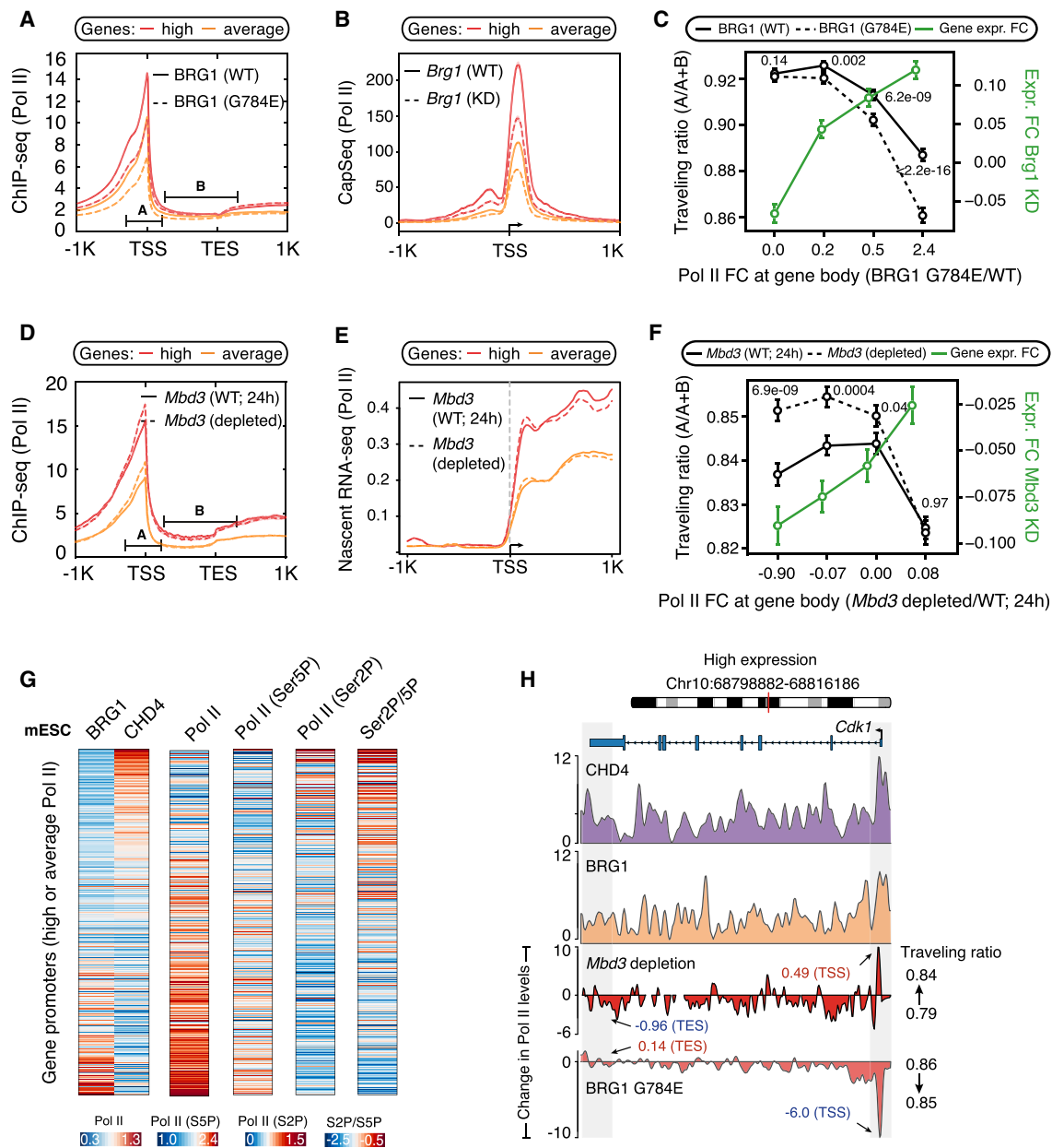
Figure 3. Differential effects of SWI/SNF and NuRD on RNA Pol II release kinetics at promoters of average/high Pol II-bound genes. (A, B) Changes in Pol II occupancy (A) and nascent RNA levels (B) at promoters (N = 6387) upon loss of BRG1 activity. Standard error is represented by a shaded area around the lines. (C) Genes with average/high Pol II promoter occupancy in mESCs (N = 6387) are binned into four groups (1597 genes each) based on the changes in the levels of Pol II released into the gene body upon loss of BRG1 activity (x-axis). For each bin, the changes in traveling ratio (solid vs. dashed black lines) and gene expression (green line) upon loss of BRG1 activity are shown (Wilcoxon rank-sum test, two-sided). (D–F) Same as A–C but following Mbd3 loss. (G) Genes (N = 6387) are binned into groups of 25 each based on the CHD4 and BRG1 binding ratio at their promoters. For each group, the median occupancy levels of initiating (Ser5p) and elongating (Ser2p) Pol II forms are shown. (H) Genome browser view for Cdk1 , where loss of BRG1 activity leads to a decrease in Pol II promoter occupancy. The opposite is observed following Mbd3 depletion.
