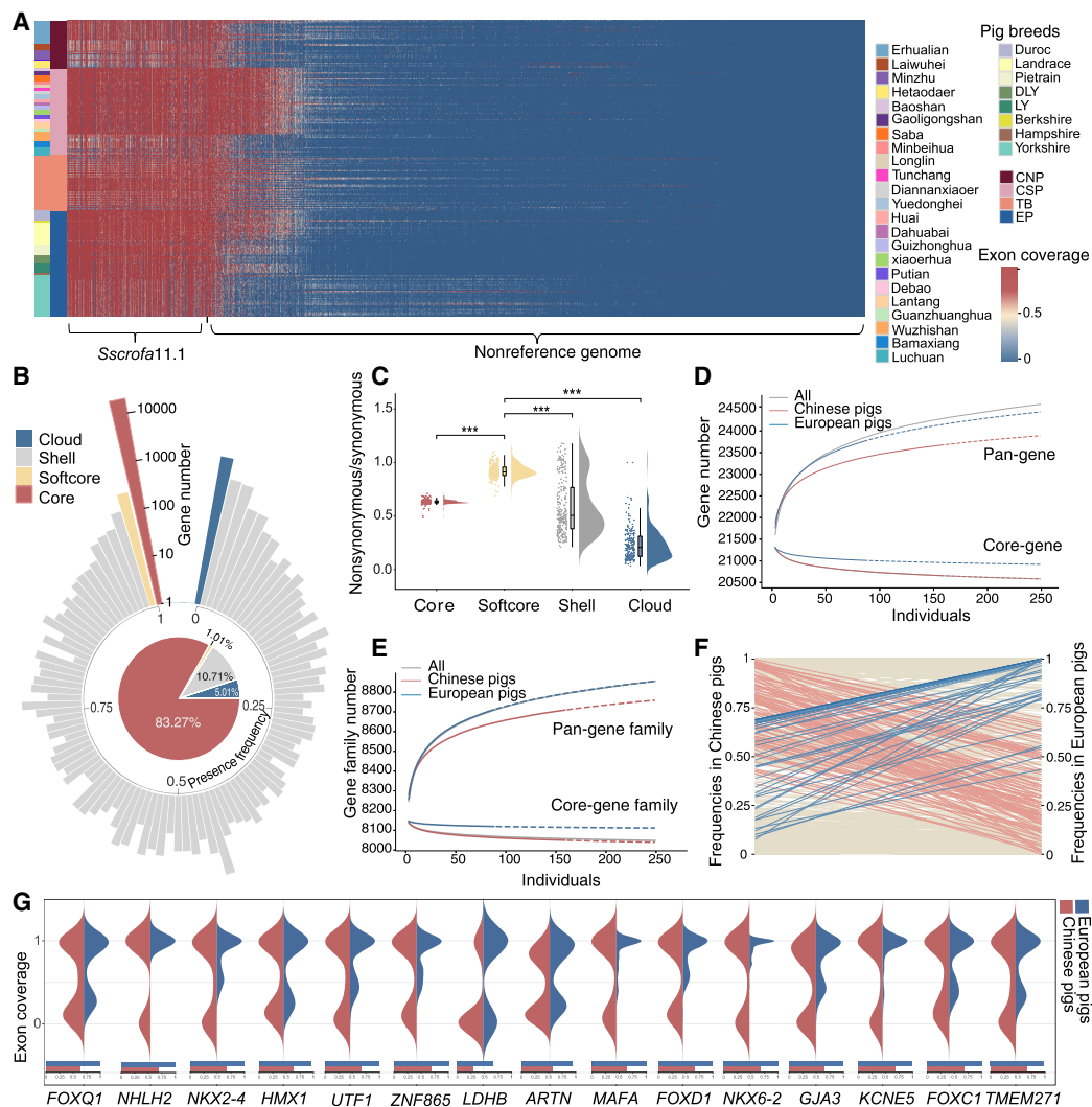
Figure 2. Characterization of gene PAVs. (A) The heatmap illustrates the exon coverage of dispensable genes identified in the reference genome S. scrofa 11.1 and nonreference genome sequences. The colors listed on the left side of the heatmaps represent different pig breeds. (B) The circle histogram depicts the distribution of gene counts with different presence frequencies in the pig population. The pie chart shows the proportion of core, softcore, shell, and cloud genes in the pig genic pangene. (C) The ratio of nonsynonymous SNPs to synonymous SNPs in core, softcore, shell, and cloud genes. Significance values were calculated: (***) P < 1 \times 10^{-6} , Wilcoxon test. (D) Saturation curve modeling the genic pangene and core-genome size in Chinese pigs, European pigs, and 250 individuals. The solid curve denotes fitting to the maximum gene number of sampled individuals, and the dashed curve depicts the extrapolation of the fitting. (E) Modeling of gene families in the pangene and core genome. (F) The left y-axis and the right y-axis are occurrence frequencies of dispensable genes in Chinese pigs and European pigs, respectively. Pink and blue lines denote the genes that are favorable for Chinese pigs and European pigs, respectively. Light brown lines denote the genes with a change of presence frequency that is less than 0.4 between the two populations. (G) Comparison of probability distribution for exon coverage among populations of Chinese and European pigs for 15 genes having higher presence frequency in European pigs. The blue and red bars denote the presence frequencies of the dispensable genes in Chinese pigs and European pigs, respectively.
