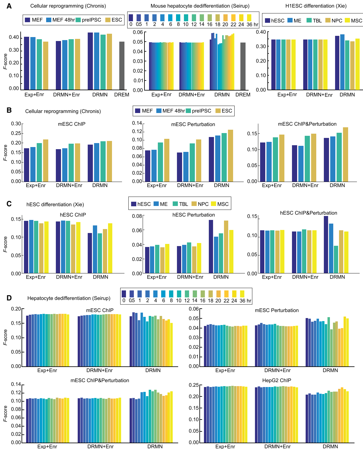
Figure 3. Performance of regulator ranking and inferred networks of DRMN. (A) The F -score of regulator ranking with different strategies for cellular reprogramming, mouse hepatocyte dedifferentiation, and H1ESC differentiation. Each plot shows regulator enrichment of expression-based modules (Exp + Enr), regulator enrichment of DRMN modules (DRMN + Enr), regulator ranking based on inferred DRMN networks (DRMN), and regulator ranking from DREM (when applicable). (B) F -score-based performance of inferred networks and baseline networks for cellular reprogramming, when compared to ChIP-based, perturbation-based, and intersection of the ChIP and perturbation-based gold standards in mESCs. (C) F -score-based performance of inferred networks and baseline networks for H1ESC differentiation, when compared to ChIP-based, perturbation-based, and intersection of the ChIP- and perturbation-based gold standards in hESCs. (D) F -score-based performance of inferred networks and baseline networks for mouse hepatocyte dedifferentiation, when compared to ChIP-based, perturbation-based, and intersection of the ChIP- and perturbation-based gold standards for mESCs, as well as the ChIP-based gold standard from the HepG2 cell line. In each panel, we show the baseline networks from regulator enrichment of expression-based modules (Exp + Enr), regulator enrichment of DRMN modules (DRMN + Enr), and inferred networks with edges scored by input feature multiplied by estimated regression coefficients (DRMN).
