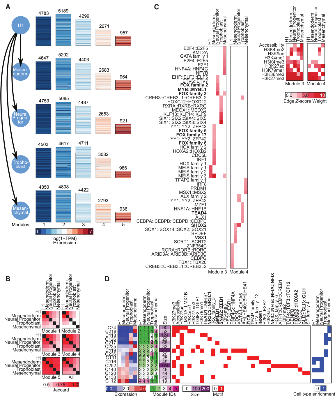
Figure 6. Application of DRMN to ESC differentiation data set using histone marks, accessibility, and Q-motifs. (A) Shown are gene expression ( \log 1 + \text{TPM} ) patterns of the k=5 modules for each lineage (major row). The number above the heatmap is the number of genes in that module. The color corresponds to the level of expression, with more red denoting high expression and more blue denoting low expression. (B) Similarity of modules across lineages as measured by Jaccard index. The color intensity is proportional to the module match. (C) Inferred regulators for each module across time. Only modules with highest expression (3 and 4) and that had TFs as regulators are shown. The red intensity is proportional to the z-score significance of the regression weight of a regulator. For all values, see Supplemental Table S6. (D) Selected transitioning gene set profiles showing changes into the high expression modules (3, 4, 5). Shown are the mean expression levels of genes in the gene set (left; red–blue heatmap), the module assignment (second), the number of genes in each module (third), the set of regulators for each gene set (white–red heatmap), and enrichment in lineage-specific gene sets from Xie et al. (2013). The complete transitioning gene set is shown in Supplemental Figure S14. Some of the regulator names were shortened for space; the full names are available in Supplemental File S7. Bolded names are those discussed in the text.
