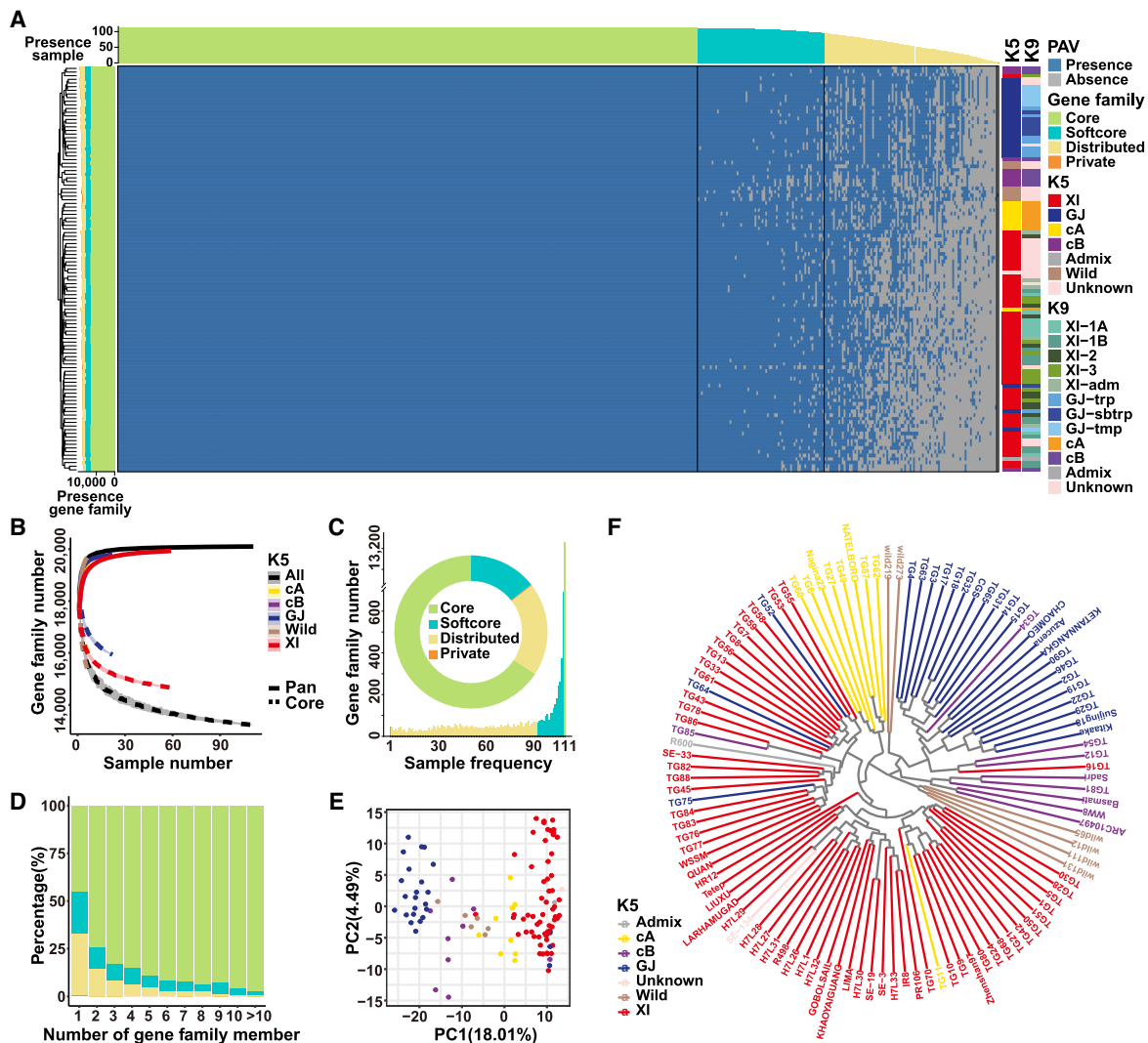
Figure 2. Gene family PAVs in 111 rice accessions. (A) Heat map of gene family PAVs of 111 rice accessions. (B) The pan-genome size estimation using 111 rice accessions for all rice accessions and subpopulations (All, Wild, XI, cA, GJ, cB). (C) The sample numbers and percentages of core, softcore, distributed, and private gene families. (D) The percentage of core, softcore, distributed, and private members in gene families. (E) The PCA analysis of 111 rice accessions using gene family PAVs. (F) The clustering of 111 rice accessions using gene family PAVs.
