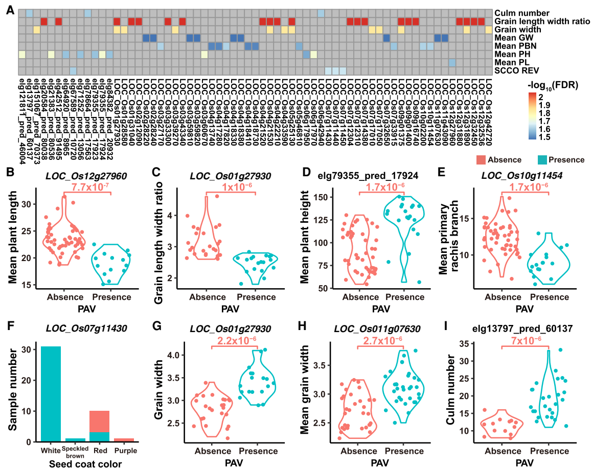
Figure 5. The associations between phenotypes and gene PAVs. (A) The association heat map of gene PAVs and phenotypes (only associations with P < 1 \times 10^{-5} and \text{FDR} < 5 \times 10^{-2} are displayed). (Mean GW) mean grain width, (Mean PBN) mean primary rachis branch, (Mean PH) mean plant height, (Mean PL) mean plant length, and (SCCO REV) seed coat color. The phenotypes started with “mean” are measured in this research. (B–I) Some examples of gene PAVs significantly associated with phenotypes: (B) Mean plant length and LOC_Os12g27960 ( P = 7.7 \times 10^{-7} , \text{FDR} = 2.5 \times 10^{-2} ); (C) Grain length width ratio and LOC_Os01g27930 ( P = 1.0 \times 10^{-6} , \text{FDR} = 8.2 \times 10^{-3} ); (D) Mean plant height and a predicted gene elg79355_pred_17924 ( P = 1.7 \times 10^{-6} , \text{FDR} = 1.7 \times 10^{-2} ); (E) Mean primary rachis branch and LOC_Os10g11454 ( P = 1.7 \times 10^{-6} , \text{FDR} = 2.3 \times 10^{-2} ); (F) Seed coat color and LOC_Os07g11430 ( P = 2 \times 10^{-6} , \text{FDR} = 2.1 \times 10^{-2} ); (G) Grain width and LOC_Os01g27930 ( P = 2.2 \times 10^{-6} , \text{FDR} = 1.3 \times 10^{-2} ); (H) Mean grain width and LOC_Os11g07630 ( P = 2.7 \times 10^{-6} , \text{FDR} = 3.2 \times 10^{-2} ); (I) Culm number and a predicted gene elg13797_pred_60137 ( P = 7.0 \times 10^{-6} , \text{FDR} = 2.3 \times 10^{-2} ).
