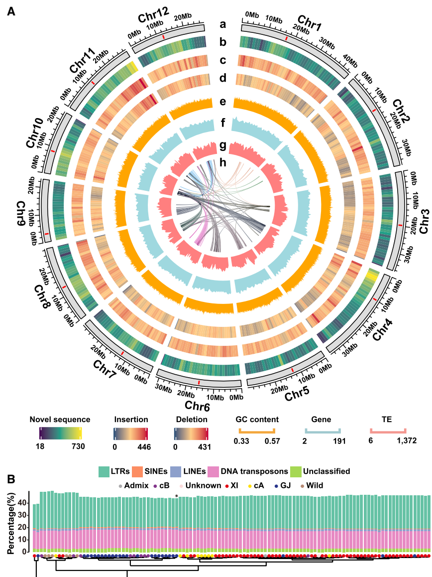
Figure 1. Genomic features of the rice pan-genome derived from 111 rice accessions. (A) A Circos display of the rice pan-genome. From outer to inner circles, they stand for (a) chromosomes (centromeres are in red), (b) novel sequences distributions, (c) insertion and (d) deletion distributions ( \geq 50 bp), (e) GC content distributions (orange), (f) gene distributions (blue), (g) transposable element distributions (light red), and (h) frequent translocation regions ( \geq 20 translocation events in 1 Mb). (B) Composition of transposable elements in terms of the percentages of the genome size in the 111 rice accessions. (*) NipRG.
