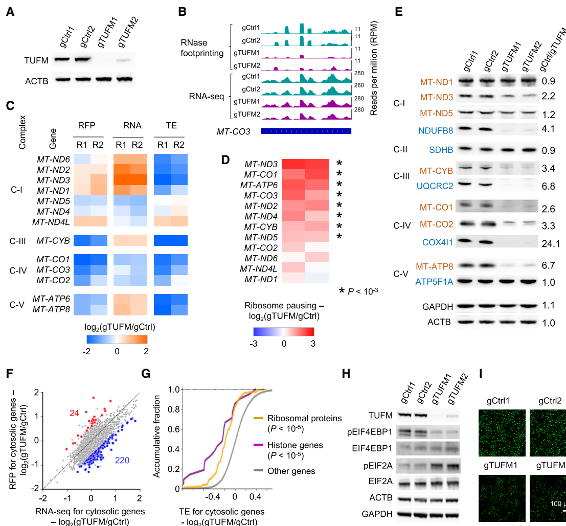
Figure 4. Regulation of mitochondrial and cytosolic RNA translation after TUFM knockout. (A) The western blots showing TUFM knockout. The expression of actin (ACTB) was used as the control. (B) RNase footprinting and RNA-seq read distribution across the MT-CO3 gene in TUFM knockout and control cells. (C) The regulation of ribosome occupancy (ribosome footprints [RFP]), RNA expression (RNA), and translation efficiency (TE) of 13 mitochondria-encoded genes after TUFM knockout. (R1/R2) Replicates 1 and 2. Complexes of the mitochondrial electron transport chain are indicated at left (I, III, IV, and V). (D) The regulation of ribosome pausing of mitochondria-encoded genes after TUFM knockout. The ribosome pausing level was calculated as the ratio of RNase footprinting read density in the first 20% of a transcript versus the remaining. Asterisks indicate significantly increased ribosome pausing after TUFM knockout with a Fisher's exact test ( P < 10^{-3} ). (E) Western blots showing the expression of mitochondria-encoded (red) and nuclear-encoded (blue) mitochondrial proteins after TUFM knockout. The expression levels of GAPDH and ACTB were used as the control. The ratios of protein expression between the control and TUFM knockout are shown. Complexes I–V of the mitochondrial electron transport chain are indicated at left. (F) Change in mRNA and RFP levels after TUFM knockout. The genes showing differential translation efficiency are highlighted. (Blue) Down-regulated; (red) up-regulated. (G) The cumulative distribution function plot showing the changes in TE of indicated gene sets. The P -values comparing “ribosome proteins” and “histone genes” versus other genes are shown. (H) Western blots showing the expression of translation factors after TUFM knockout. (I) Nascent proteins containing the methionine analog (AHA) were visualized by fluorescence microscopy. An identical setting was used to acquire images, and the percentage of fluorescent cells was 100%. The down-regulation of AHA fluorescence in TUFM knockout cells indicates the inhibition of new protein synthesis.
