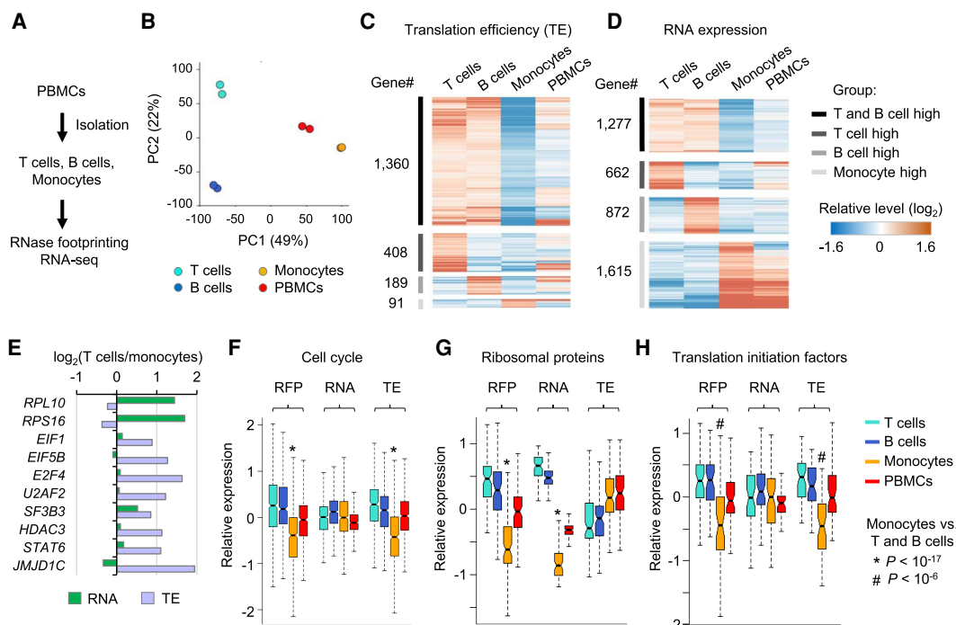
Figure 6. Regulation of RNA translation across human primary immune cell types. (A) Experimental steps to isolate T cells, B cells, and monocytes from PBMCs and then perform RNase footprinting and RNA-seq. (B) The principal component analysis (PCA) of ribosome occupancies of T cells, B cells, monocytes, and PBMCs. Genes showing more than twofold regulation across cells were used in the analyses. The percentages of variance explained by PC1 and PC2 are shown in parentheses. (C,D) The heatmap showing genes with regulation of translation efficiency (C) and RNA expression (D) comparing T cells, B cells, and monocytes. (E) Example genes showing differential RNA expression and translation efficiency, comparing T cells versus monocytes. (F–H) Boxplots showing the relative levels of ribosome occupancy (RFP), RNA expression, and translation efficiency (TE) for indicated genesets comparing T cells, B cells, monocytes, and PBMCs: “cell cycle” (F), “ribosomal proteins” (G), and “translation initiation factors” (H). The * or # label indicates the Wilcoxon rank-sum test P -value showing the geneset has significantly lower expression in monocytes, compared with both T cells and B cells.
