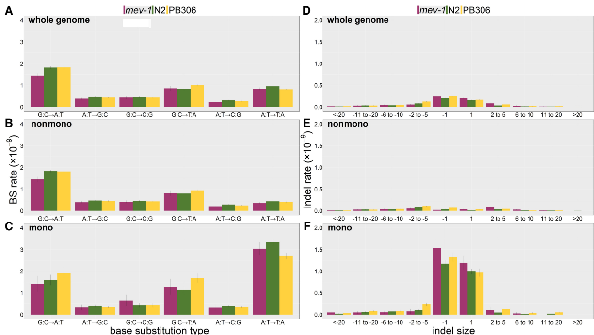
Figure 2. Mutation rates. (A–C) Type-specific base-substitution rates, by strain. (D–F) Size-specific indel rates, by strain. (A,D) Genome-wide mutation rates; (B,E) rates at nonmononucleotide repeat sequence; (C,F) mononucleotide repeat sequence. All rates are scaled as 10^{-9} per base per generation; note the difference in y-axis scale between panels A–C and panels D–F. Error bars, one SEM.
