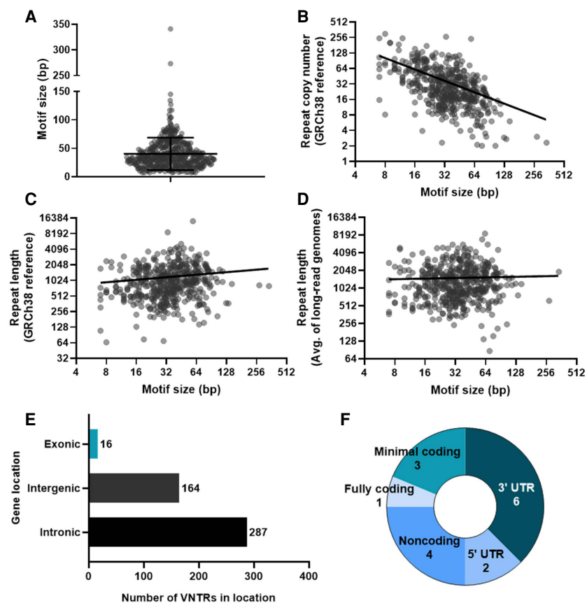
Figure 1. Characterization of 467 human-specific VNTR expansions assessed. (A) Violin plot of motif size for each VNTR. Lines show mean (40.1 bp) and standard deviation ( \pm 28.6 bp). (B) Scatter plot of motif size versus repeat copy number in the GRCh38 human reference genome. Axes are \log_2 and line is log-log (best-fit slope = -0.74). (C) Scatter plot of motif size versus total repeat length in the GRCh38 human reference genome. Axes are \log_2 and line is log-log (best-fit slope = 0.16). (D) Scatter plot of motif size versus average total repeat length in eight SMRT long-read sequenced genomes representing different superpopulations. Axes are \log_2 and line is log-log (best-fit slope = 0.034). (E) Bar chart summarizing overall VNTR locations in the genome. (F) Pie chart breaking down specific locations of VNTRs in exons.
