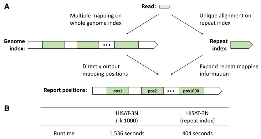
Figure 1. Repeat index enables faster 3-nt read alignment. (A) HISAT-3N aligns reads using two different strategies: (1) HISAT-3N can directly align reads to the whole genome using the genome index and output their mapped locations (A, left), and (2) HISAT-3N can use a repeat index to uniquely align reads to the repeat sequences regardless of how many locations to which they align on the genome (A, right). (B) Runtime comparison between direct mapping and repeat mapping strategy. The test data are 10 million simulated single-end BS-seq reads (0.2% per-base sequencing error rate).
