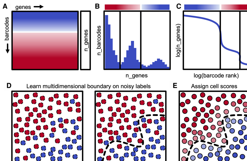
Figure 2. Description of dropkick filtering method. (A) Diagram of scRNA-seq counts matrix with initial cell confidence for each barcode based solely on total genes detected ( n_genes ), depicted by color (red, empty droplet; blue, real cell). (B) Histogram showing the distribution of barcodes by their n_genes value. Black lines indicate automated thresholds for training the dropkick model. (C) \log(n\_genes) versus \log(\text{rank}) representation of barcode distribution as in dropkick QC report (Fig. 1A). Thresholds from B are superimposed. (D) Thresholds in heuristic space (B, C) are used to define initial training labels for logistic regression. (E) dropkick chooses an optimal regularization strength through cross-validation and then assigns cell probabilities and labels to all barcodes using the trained model in gene space.
