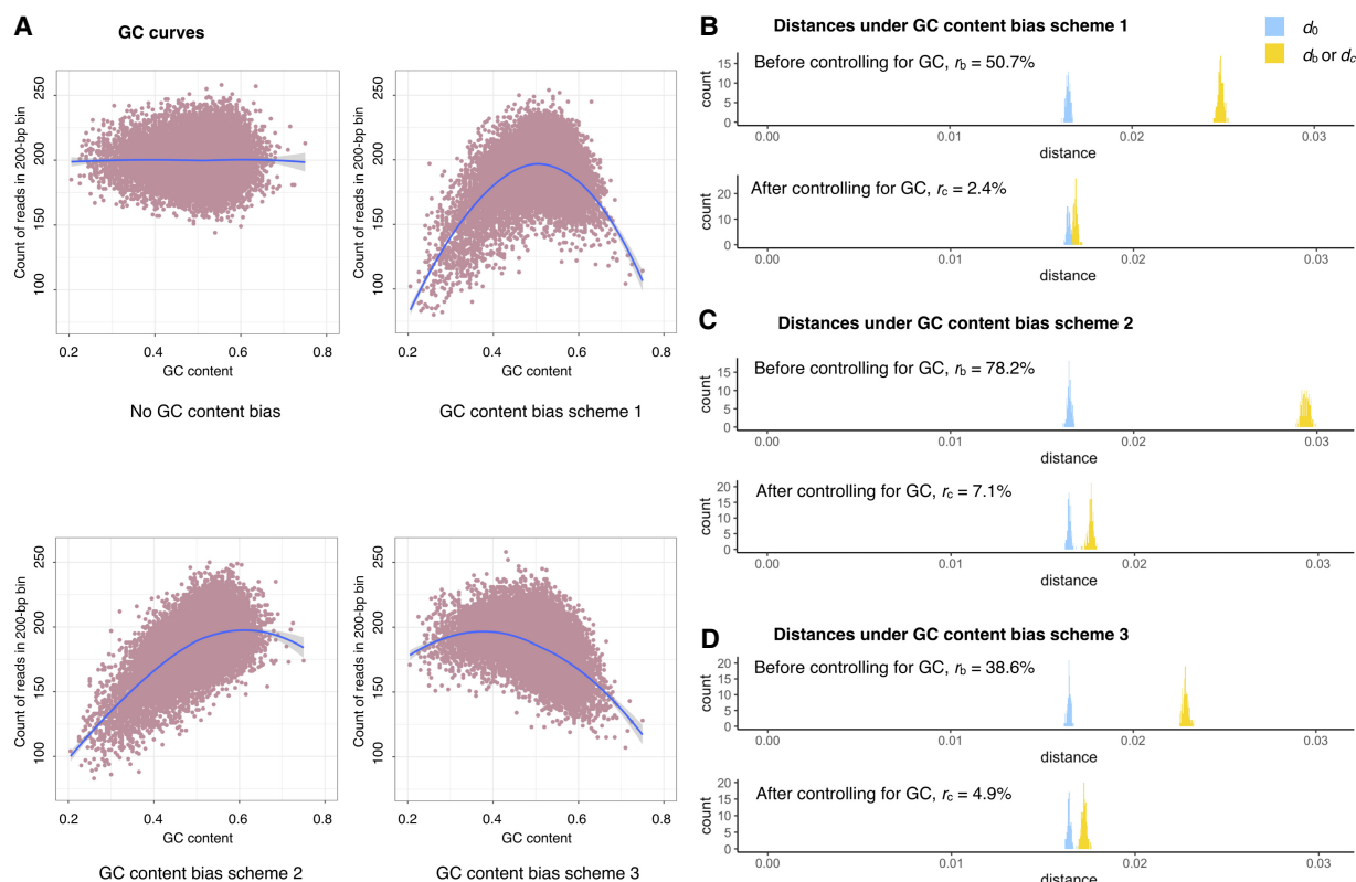
Figure 4. The effect of controlling for GC content bias in Nubeam. (A) GC content (x-axis) versus bin coverage (y-axis) to demonstrate patterns of GC bias for three simulation schemes, with LOESS curve marked in blue. Recall that r_b = (\bar{d}_b - \bar{d}_0) / \bar{d}_0 and r_c = (\bar{d}_c - \bar{d}_0) / \bar{d}_0 measure relative differences before and after controlling for GC bias, respectively. (B) r_c = 2.4\% after controlling for GC bias versus r_b = 50.7\% before controlling for GC bias for simulation scheme 1. (C) r_c = 7.1\% after controlling for GC bias versus r_b = 78.2\% before controlling for GC bias for simulation scheme 2. (D) r_c = 4.9\% after controlling for GC bias versus r_b = 38.6\% before controlling for GC bias for simulation scheme 3.
