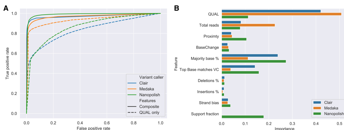
Figure 2. Random forest-based variant filtering using Nanopolish, Medaka, and Clair. (A) Receiver operating characteristic (ROC) curve for random forest classifier using different features including Quality (QUAL only, dashed line) and a composite selection of input features (Composite, solid line) for Nanopolish (green), Medaka (orange), and Clair (blue). AUC for each variant caller: Nanopolish 0.86 to 0.98, Medaka 0.93 to 0.97, Clair 0.84 to 0.97, using QUAL and Composite features, respectively. (B) Bar chart of feature importance for composite selection of features used to train the classifier.
