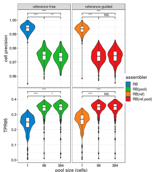
Figure 4. Cell precision and true positive rate of RNA-Bloom's reference-free and reference-guided modes over 384 cells. The simulated data set of 384 cells is split into four smaller subpools of 96 cells and 1 cell. Pool size of 1 refers to no pooling between cells. Each subpool is assembled separately, and the cell precision of the assembled isoforms in each cell is calculated based on the I95. True positive rate was calculated based on I95, denoted as TPR95. Distributions of cell precision and TPR95 were measured over all 384 cells. The comparison bars on top between different pool sizes indicate statistical significance of the difference between distributions at P < 0.001 (***), P < 0.01 (**), P < 0.05 (*), or no significance (NS) using the Wilcoxon test.
