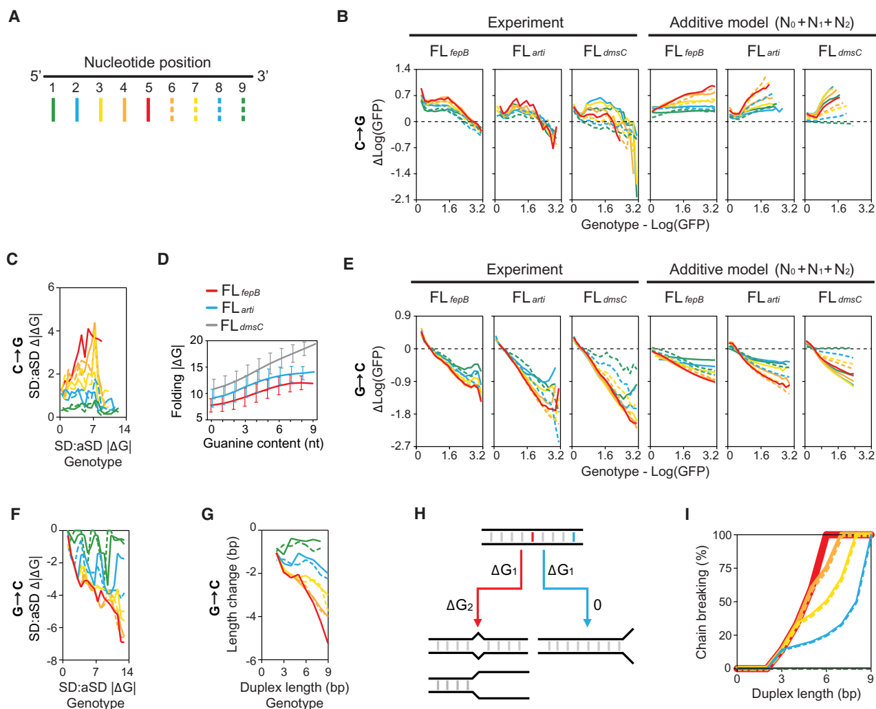
Figure 6. Global spectrum of mutational effects. (A) Markers of nucleotide positions. (B, C) Relationship between the fitness ( \text{Log}[\text{GFP}] ) (B) and SD:aSD base-pairing energy ( \Delta G ) (C) of genotypes and the effects of C→G mutations. (D) Relationship between the guanine content of SD and the RNA folding energy ( \Delta G ) of 30-nt RBS. Genotypes are ranked by the guanine content and grouped into 10 bins. Lines and bars indicate group means and standard deviations, respectively. (E–G) Relationship between the fitness (E), SD:aSD base-pairing energy (F), and SD:aSD duplex length (G) of genotypes and the effects of G→C mutations. (B, C, E–G) Genotypes are ranked by the considered phenotypes and grouped into 20, 20, 20, 20, and 10 equal-sized bins, respectively. For each phenotype-ranked group, the mean phenotypic effects of mutations at each nucleotide position in SD are computed and shown by lines styled according to A. (C, D, F) The predictions of \Delta G are \leq 0 and shown as absolute values for simplicity. (B, E) The additive model predicts mutational effects based on the fitness contribution of RBS contexts ( N_0 ), single nucleotides ( N_1 ), and pairwise epistasis ( N_2 ). (H) Chain-breaking model. Mismatch mutations occurring at the internal (red) and the edge (blue) of a RNA duplex are highlighted: ( \Delta G_1 ) energy penalty caused by base-pairing mismatches; ( \Delta G_2 ) energy penalty caused by breaking the base-pairing chain. (I) Probability of chain-breaking mutations as a function of the nucleotide position and the duplex length formed by two 9-nt position-aligned RNA strands made of any sequences. The chain-breaking probability at each nucleotide position is shown by lines styled according to A.
