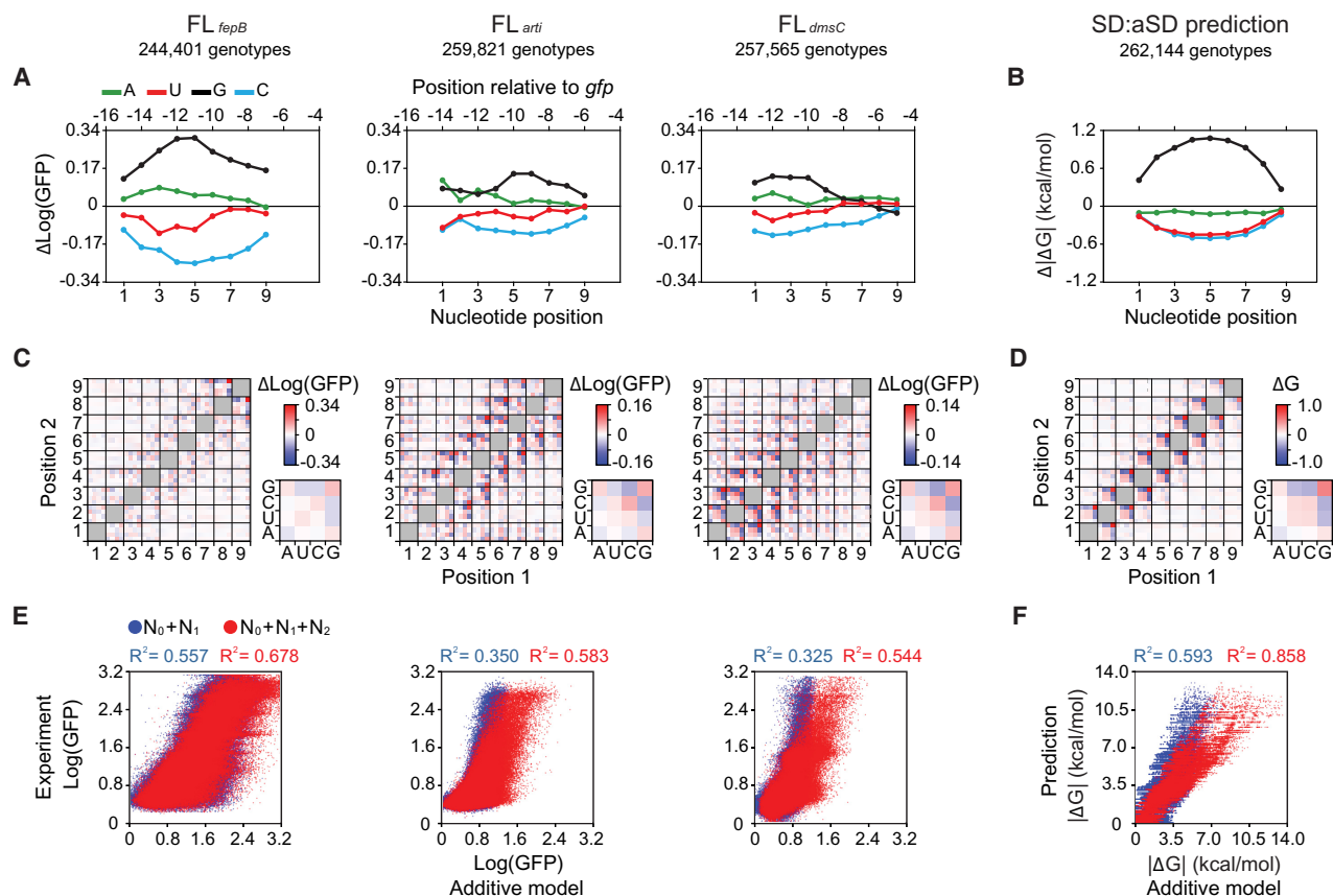
Figure 5. Fitness contribution of single nucleotides and pairwise epistasis. (A,B) Mean effects of single nucleotides on fitness ( \text{Log[GFP]} ) (A) and SD:aSD base-pairing energy ( \Delta G ) (B). (C,D) Mean effects of pairwise epistasis on fitness (C) and SD:aSD base-pairing energy (D). Color bars, large heatmaps, and small heatmaps show measurement scales, nucleotide–nucleotide epistasis across the SD sequence, and the averaged patterns of epistasis between each nucleotide position and its two upstream and two downstream neighbors, respectively. (E,F) Explanatory power ( R^2 ) of the RBS context ( N_0 ), single nucleotides ( N_1 ), and pairwise epistasis ( N_2 ) on fitness (E) and SD:aSD base-pairing energy (F). (B,D,F) \Delta G (predicted values \leq 0 ) is shown as absolute values for simplicity.
