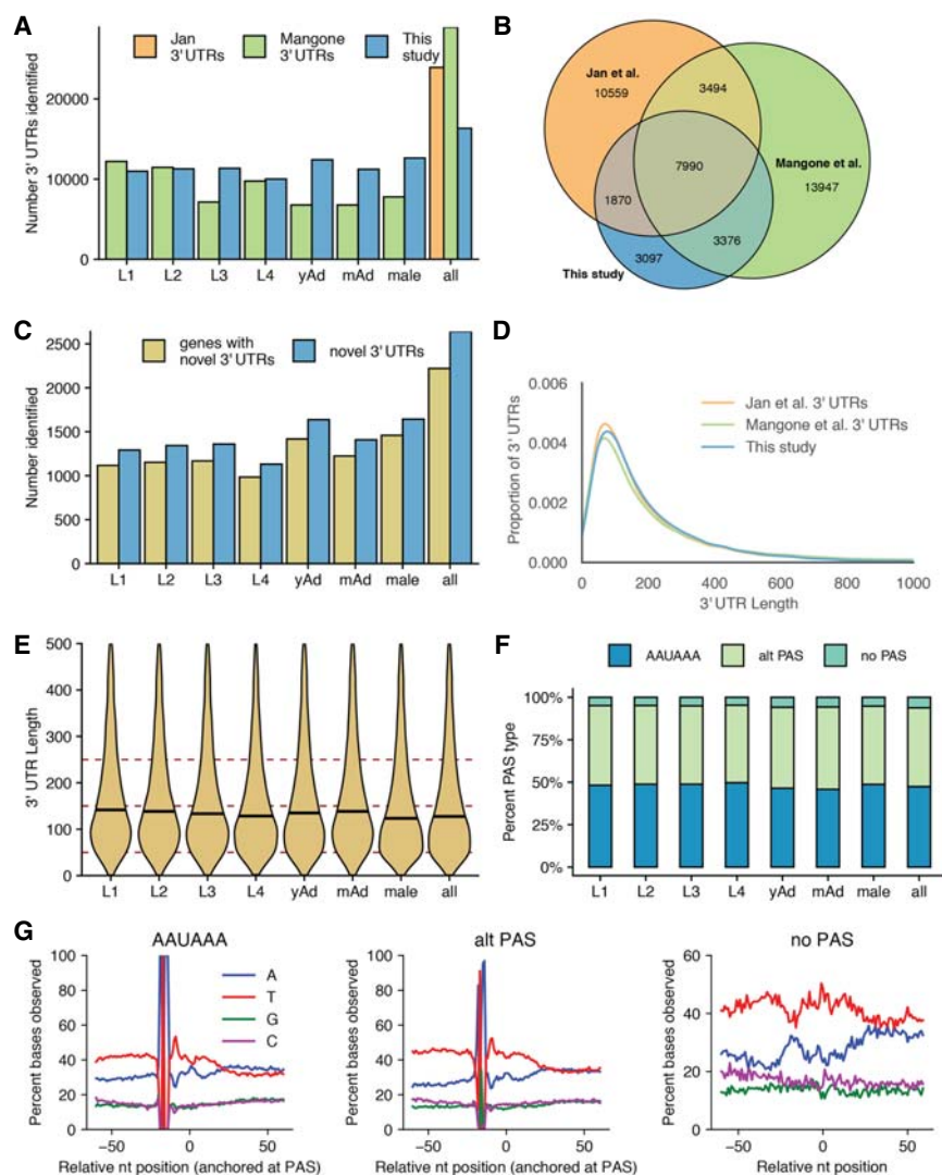
Figure 3. Properties of 3' UTRome (A) Number of 3' UTRs observed across all stages, as compared to Mangone et al. (2010) and Jan et al. (2011). (B) Venn diagram showing overlap between 3' UTRs identified in this study, Jan et al., and Mangone et al. (C) Number of novel 3' UTRs and genes with novel 3' UTRs identified in each stage and across all stages. (D) Kernel density estimate plot of 3'-UTR lengths from this study, Jan et al., and Mangone et al. (E) Violin plots showing 3'-UTR length distributions across all stages. Horizontal black lines show the median of each stage. (F) Stacked bar chart showing percentage of UTRs with the specified polyadenylation signal (PAS) across all stages. (G) Nucleotide distributions around putative PAS sites and putative cleavage sites. Canonical PAS (AAUAAA) and alternative PAS (alt PAS) distributions are anchored with the putative PAS hexamer at -19 nt. The distribution of UTRs with no PAS is anchored with the putative cleavage site at 0.
