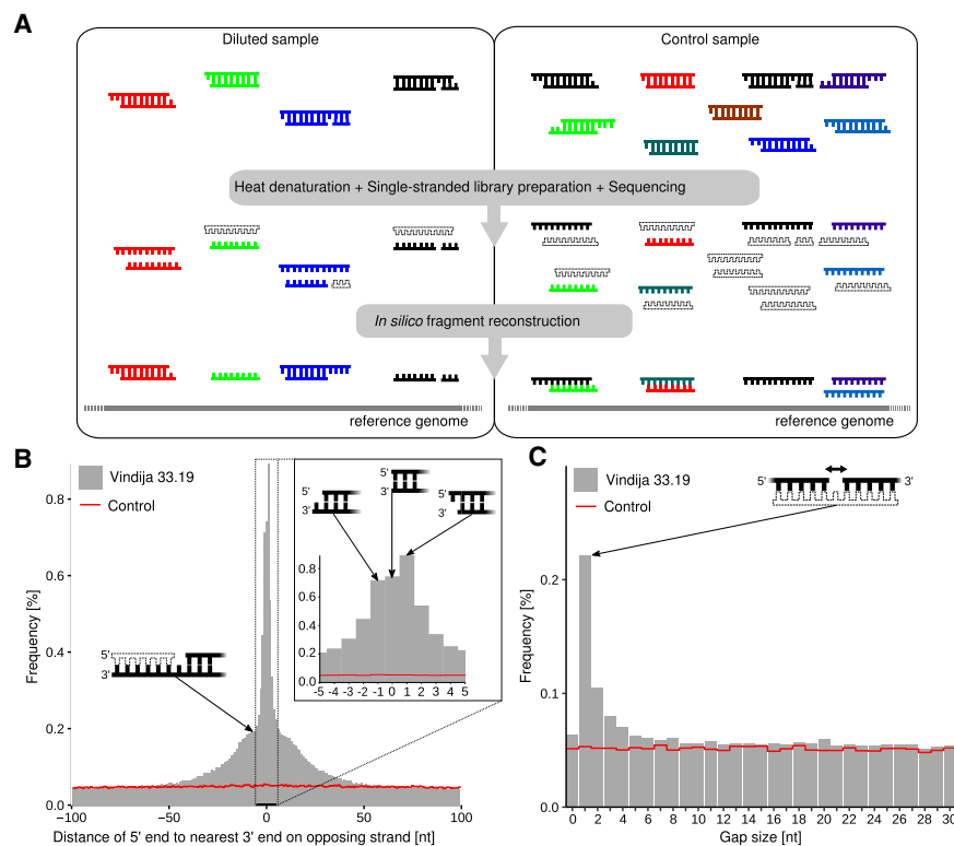
Figure 1. Identification of sequences from DNA strands originating from the same double-stranded DNA molecules. (A) Schematic overview of MatchSeq: DNA fragments isolated from ancient or recent biological material are diluted to a relatively small number, denatured by heat, converted into a single-stranded library, amplified, and deeply sequenced. Double-stranded fragments are then reconstructed in silico by identifying overlapping sequences mapping to the reference genome in reverse complementary orientation or in close proximity on the same strand. Sequences <35 bp cannot be confidently mapped to the reference and are discarded. The same analysis is performed for an equal number of control sequences obtained from shallow sequencing of a vast amount of artificially fragmented modern human DNA, in which sequences are expected to be distributed randomly across the reference genome. (B) Distribution of distances between the 5' end of each sequence to the nearest 3' end on the opposing strand obtained from Neanderthal DNA (Vindija 33.19; gray bars) and the control (red line). (C) Distribution of distances between sequence alignments on the same strand. Molecular structures putatively underlying the observed signals are indicated by schematic drawings. Filled DNA strands indicate sequences that were recovered; unfilled strands are hypothesized to be present but were not sequenced.
