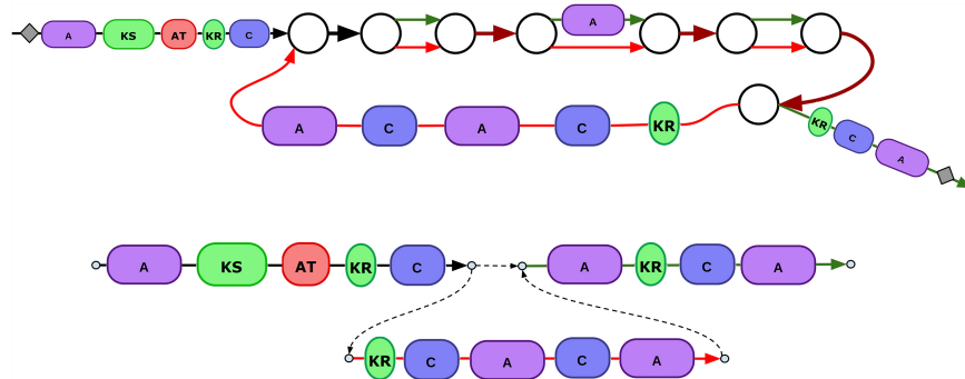
Figure 4. biosyntheticSPAdes assembly of the hectochlorin BGCs (the CYANO data set). ( Top ) The subgraph of the assembly graph corresponding to the hectochlorin BGC. metaSPAdes assembly results in four scaffolds shown by a red path, a green path, and two black edges. The repeat edges traversed by both red and green scaffolds are shown by the brown color. The domain restoration procedure had no effect on this graph. ( Bottom ) The scaffolding graph of the hectochlorin BGC has only one rural postman route that revealed the correct domain order.
