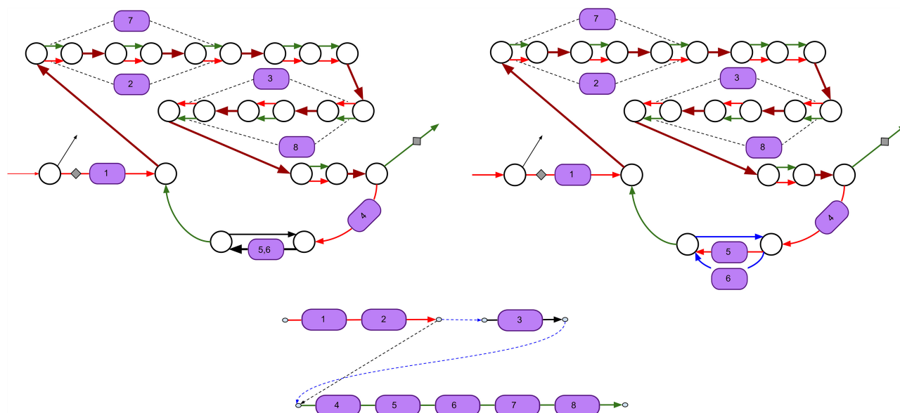
Figure 3. Subgraph of the assembly graph of Pseudomonas protegens Pf-5 corresponding to the pyoverdine NRP BGC. ( Top left ) The pyoverdine BGC is scattered over four scaffolds in the SPAdes assembly. Two scaffolds traversing single edges are shown by black color, and two scaffolds traversing multiple edges are shown by red and green colors. The repeat edges traversed by both red and green scaffolds are shown by brown color. Edges with low and high depth of coverage by reads are shown as thin and thick edges, respectively. Some A-domains span multiple edges (starting and ending positions of such domains are shown with dashed lines). ( Top right ) The domain restoration procedure restored two A-domains (5 and 6) in the assembly (SPAdes collapsed these domains into a single edge). Four scaffolds in the assembly graph are shown by red, green, blue, and black colors. ( Bottom ) The scaffolding graph of the pyoverdine BGC with a single rural postman route (dashed edges in this route are shown in blue).
