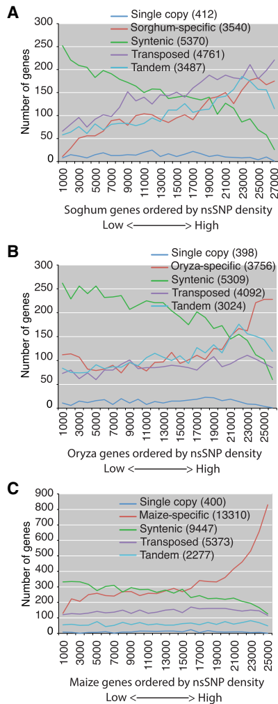
Figure 1. Number of duplicated gene types in different nsSNP density categories. All genes in (A) sorghum, (B) rice, and (C) maize are ordered by nsSNP density, ranked in 1000-gene intervals from low to high nsSNP density as shown in the x-axis.
