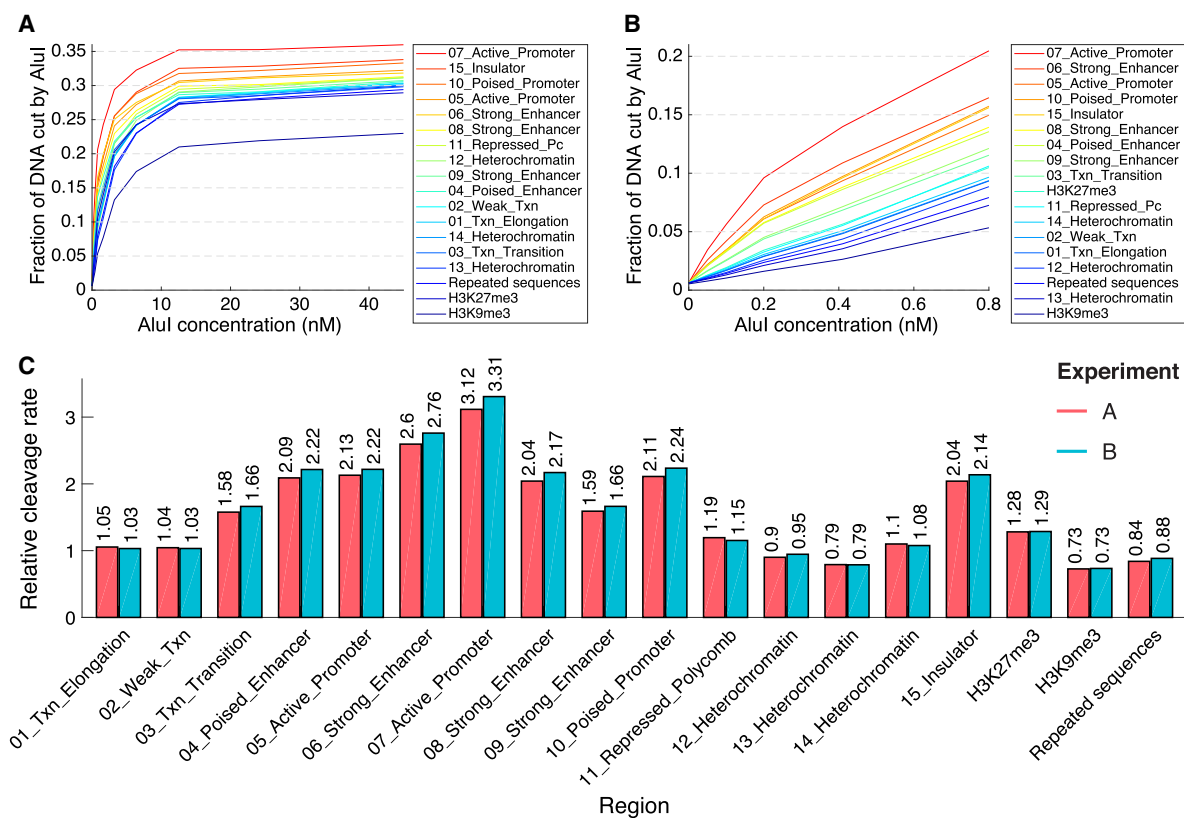
Figure 5. Heterochromatin and euchromatin have very similar DNA accessibilities in mouse hepatocytes. (A) AluI digestion kinetics for sites in the 15 epigenetic chromatin states in mouse hepatocytes defined by Bogu et al. (2016), for sites in repeated sequences (defined by RepeatMasker) and for sites marked by H3K9me3 (constitutive heterochromatin) or H3K27me3 (facultative heterochromatin) (data from Nicetto et al. 2019). (B) Initial rates of AluI digestion. (C) Quantitative comparison of initial digestion rates for the 15 epigenetic states defined by Bogu et al. (2016), repeated sequences, and regions marked by H3K9me3 or H3K27me3. Data for biological replicate experiments A and B are shown. See Supplemental Material for details of the analysis.
