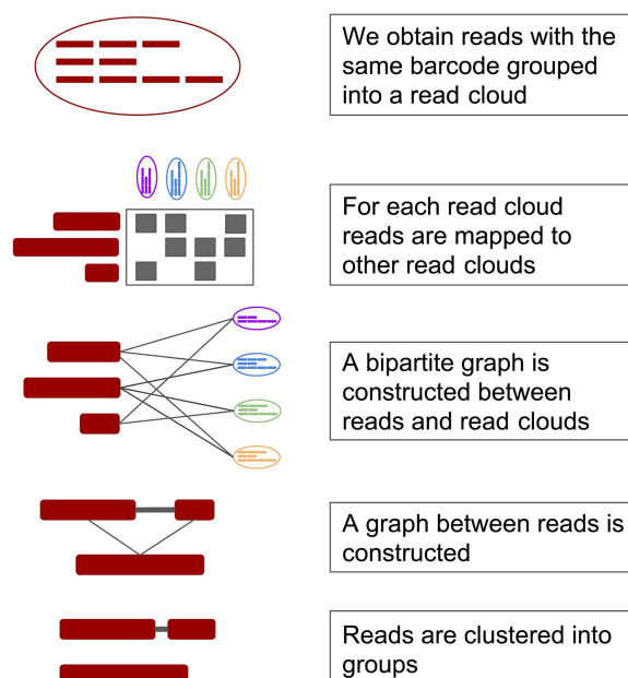
Figure 3. Processing steps for a single read cloud. From top: (1) Fragments are sequenced and tagged with 3' barcodes. (2) Reads in a given read cloud are mapped to reads in other read clouds using minimizing k -mers. (3) A bipartite graph between reads and other read clouds is constructed. (4) A graph between reads that map to the same read clouds is constructed. (5) Reads are clustered into groups.
