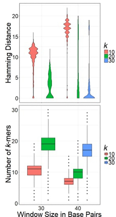
Figure 4. Top: hamming distance between windows that share minimizing k -mers, using various parameters. Bottom: number of representative minimizing k -mers per read.
