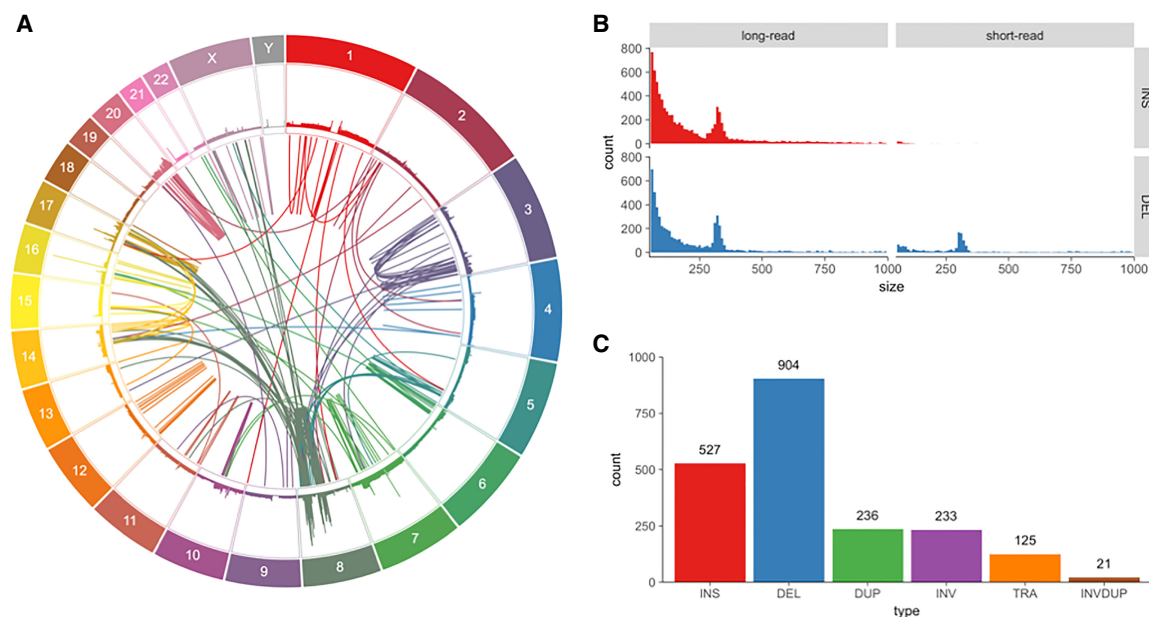
Figure 1. Variants found in SK-BR-3 with PacBio long-read sequencing. (A) Circos (Krzyszowski et al. 2009) plot showing long-range (larger than 10 kbp or inter-chromosomal) variants found by Sniffles from split-read alignments, with read coverage shown in the outer track. (B) Variant size histogram of deletions and insertions from size 50 bp up to 1 kbp found by long-read (Sniffles) and short-read (SURVIVOR 2-caller consensus) variant calling, showing similar size distributions for insertions and deletions from long reads but not for short reads, where insertions are greatly underrepresented. (C) Sniffles variant counts by type for variants above 1 kbp in size, including translocations and inverted duplications.
