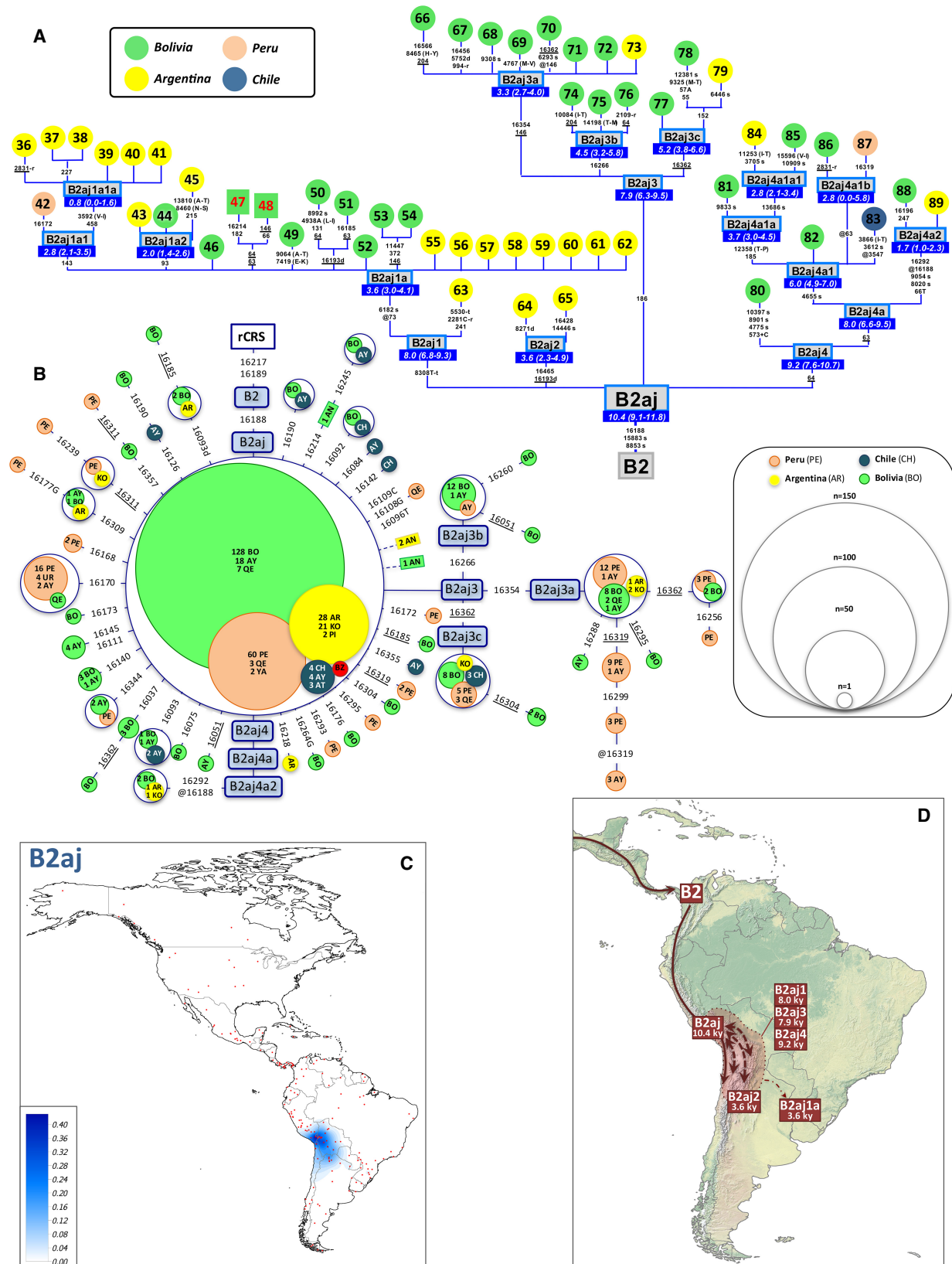
Figure 2. (A) Maximum parsimony tree of B2aj complete mitochondrial genomes. (B) Network of B2aj CR haplotypes obtained from population surveys (listed in Supplemental Table S2). (C) Interpolated frequencies of B2aj mtDNAs in America. (D) Main migration routes of B2aj as inferred from phylogeographic data. See the legend of Figure 1 for more details on the phylogenies of panels A and B.
