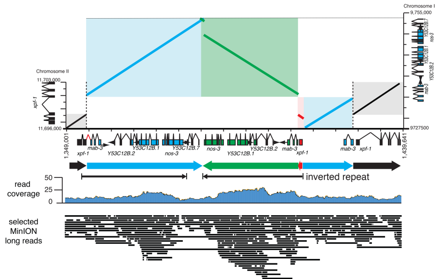
Figure 5. Delineation of complex genome rearrangements. Schematic of the xpf-1(e1487) complex mutation in contig017. The left y-axis shows the wild-type xpf-1 gene structure and the right y-axis shows the mab-3 region. The mutation is a duplication and insertion of ~20 kb of the mab-3 region in two segments into the second intron of xpf-1 (blue). The larger segment of the inserted region along with the flanking xpf-1 exon 2 has been duplicated creating an inverted repeat (green and red). Shown below is read coverage and selected MinION reads mapping to the region spanning the various breakpoints.
