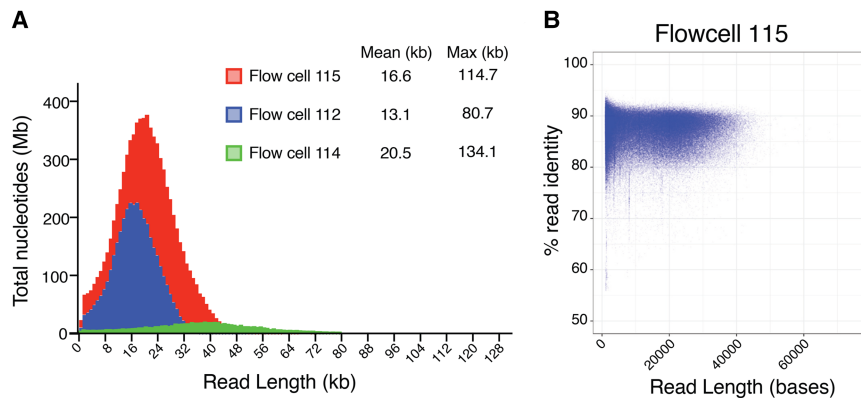
Figure 1. Summary of MinION sequence reads of the C. elegans VC2010 wild-type strain genome. (A) Histogram of read lengths from flow cells 112, 114, 115. (B) Plot of % read identity aligned to the C. elegans reference genome vs. read length from flow cell 115. Mean % identities ranged from 85.90% to 86.35% for the three flow cells (Supplemental Fig. S1).
