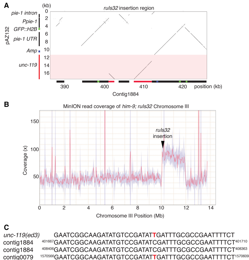
Figure 6. Delineation of an exogenous plasmid DNA array integration and duplication event. (A) Dot plot of the ruls32 insertion in contig1884 against the pAZ132 plasmid and unc-119 gene (red) that were integrated by biolistic transformation. The y-axis shows the pAZ132 plasmid structure and the unc-119 gene structure. The insertion contains three copies of GFP::H2B and two partial copies of unc-119 . (B) MinION read coverage for Chromosome III. Note the ~2-Mb duplication in the region where ruls32 has been integrated. Red line is coverage and purple shading is coverage deviation. (C) MinION-generated sequence identified the two wild-type copies of unc-119 inserted with ruls32 and the unc-119(ed3) mutation in contig0079. Superscript numbers refer to position within the contig.
