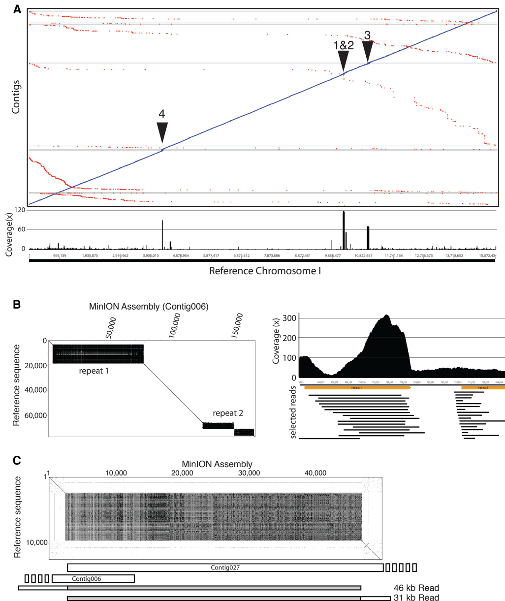
Figure 4. MinION sequencing and assembly reveals genome expansion of C. elegans repeat regions. (A) LASTZ alignment of contigs to the C. elegans reference Chromosome I. Below is a plot of coverage of the 'All data' assembly contig sequences against the reference. Note the high coverage areas (indicated as 1–4) that correlate with repeat regions. (B) (Left) Dot plot of the MinION-derived contig containing repeats 1 and 2 against the reference sequence. (Right) Plot of sequence read coverage (reads > 5 kb) in the repeat regions. Selected reads spanning the expanded repeats are shown below. Note the high coverage of repeat 1, which suggests that this repeat is even larger than predicted in the contig shown. Repeat 2 read coverage, which is similar to the average read coverage across the genome, suggests that this repeat expansion is correct. (C) Dot plot of the end termini of contig006 and contig027 against the reference sequence demonstrating the expansion of repeat 3. Two of the longest reads mapping to this repeat are shown below with the repeat highlighted in gray.
