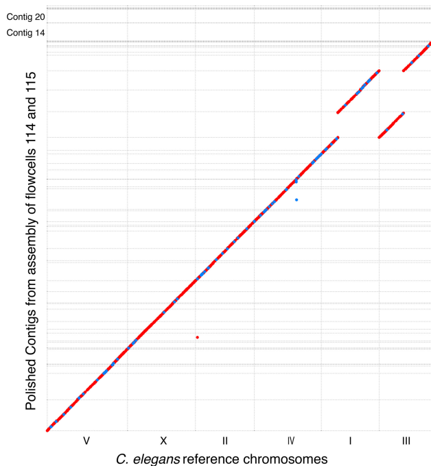
Figure 3. MinION produces high contiguity C. elegans genome assembly. MUMmer alignment plot of contigs from assembly of combined data from flow cells 114 and 115 against the C. elegans reference genome. The C. elegans chromosomes are arranged by size along the x -axis and 114 +115 contigs along the y -axis. Forward strand matches are in red and reverse strand matches are in blue. Note that the large bacterial contigs 14 and 20 do not align to the C. elegans reference genome.
