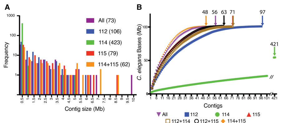
Figure 2. De novo C. elegans genome assembly from MinION-generated long reads. Comparison of Canu-generated genome assemblies for individual and combined flow cell data. (A) Distribution of contig sizes for different assemblies. Number in parentheses refers to total contigs in the assembly. (B) Plot of contig coverage of the reference genome from assemblies produced from the individual and combined flow cells. Arrows denote the number of contigs that align to the C. elegans reference genome.
