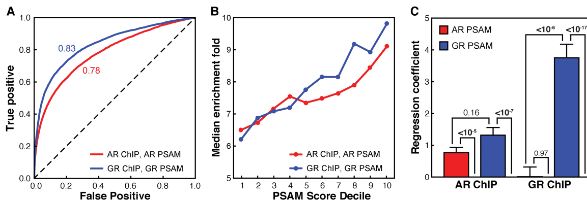
Figure 5. Differences of intrinsic specificity between AR- and GR-DBD are reflected in the respective cellular genomic binding profiles. (A) Ability of the AR (red) and GR (blue) PSAMs to identify true ChIP-seq peaks as measured by the receiver operator characteristic (ROC) of binary classifiers identifying peaks versus adjacent regions. (B) Comparison of the median enrichment over background from ChIP-seq (y-axis) to the relative affinity for the strongest sequences within the ChIP-seq peak calculated from the position specific affinity matrix for AR (red) and GR (blue). In vitro affinity is binned by decile (e.g., 10 is the sequence space representing the top 10% highest affinity sites) (C) Multiple linear regression coefficients in models that use AR (red) and GR (blue) PSAM scores to predict AR (left) and GR (right) ChIP-seq peak enrichments. P -Values were calculated using t -tests.
