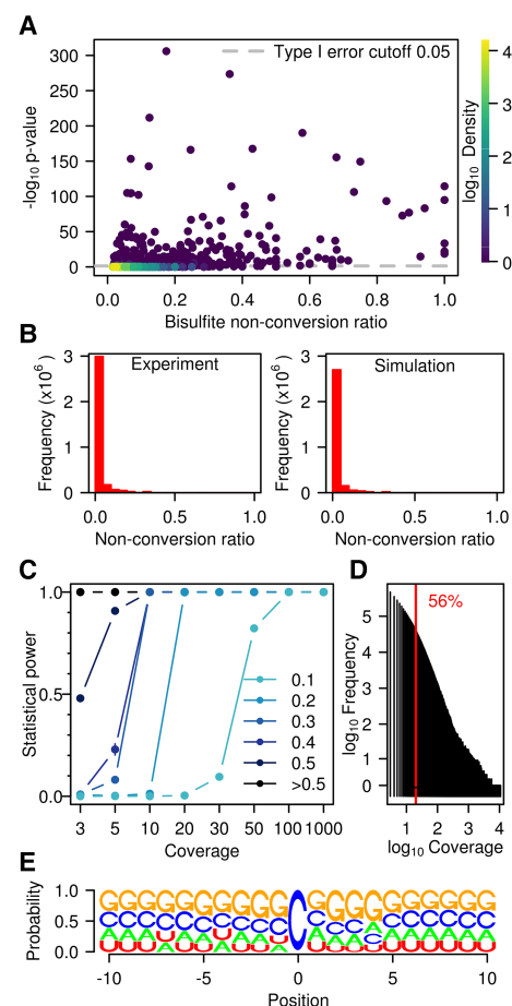
Figure 3. Statistical analysis of WTBS data sets. (A) Bisulfite nonconversion ratio (x-axis) and -\log of methylation P -values (y-axis) for 56,940 cytosines with ratio > \lambda_p/\text{coverage} that are common to the three wild-type replicates. Color indicates density (count of points per symbol area). (B) Number of cytosines and nonconversion ratios, as determined experimentally (left) or by simulation (right). (C) Statistical power stratified by coverage and by nonconversion ratio. (D) Histogram of coverage in a representative (Wt1L) sequencing data set. The red line indicates a coverage of 20x. (E) Logo plot for all cytosines with a ratio > 0.1 and significant P -value ( < 0.05 ) in at least one sample.
