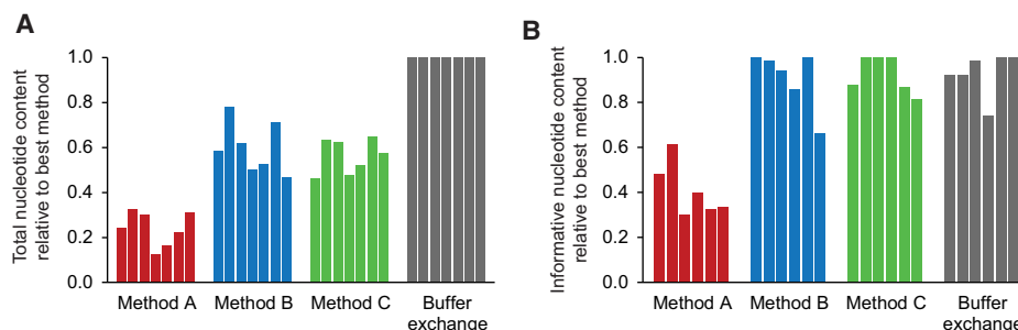
Figure 5. Sequence content of libraries obtained from extracts prepared with the four methods as inferred by qPCR and shotgun sequencing. (A) The sum of nucleotides in all library molecules relative to that of the best method. (B) The sum of ‘informative’ nucleotides in the libraries, i.e., the sum of nucleotides subsumed in library molecules \geq 35 bp that produce sequence alignments, relative to that of the best method. Numbers for the libraries prepared from buffer exchange extracts were multiplied by 2.5 to compensate for the smaller volume of lysate used.
