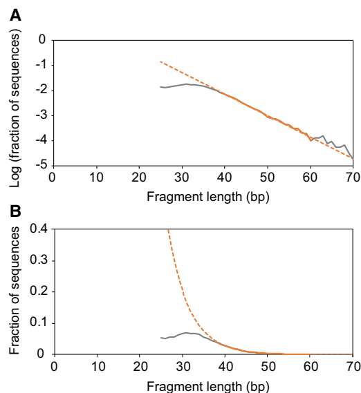
Figure 1. DNA fragment size distribution reconstructed from a hominin femur fragment from Sima de los Huesos. Sequences \geq 25 bp from putatively endogenous ancient DNA fragments were isolated from published sequence alignments to the human reference genome (Meyer et al. 2016) by requiring a signal of deamination to be present, i.e., a terminal C to T substitution, and removing alignments with substitutions other than C to T. The first filter depletes human contamination, whereas the second reduces the impact of spurious alignments of microbial sequences. (A) Log-transformed fragment size distribution. Fragment sizes between 40 and 60 bp provide the best fit to an exponential model of DNA decay (dashed line). (B) The same fragment size distribution plotted on a linear scale to visualize more clearly the underrepresentation of short DNA fragments.
